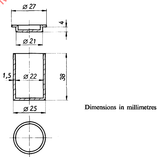
FIG. 1. — Silica crucible and lid
