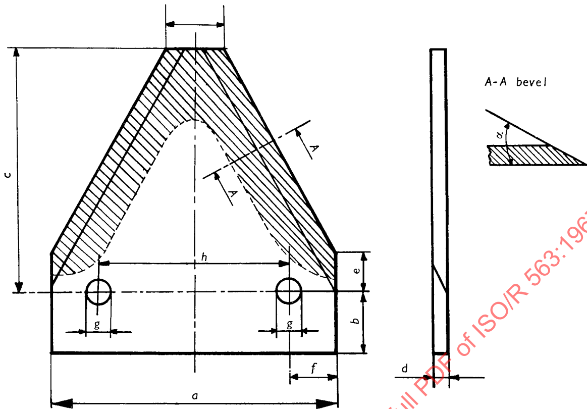
FIG. 1 — Knife dimensions
