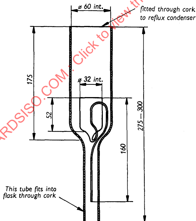
FIGURE 3 Siphon tube and adaptor
