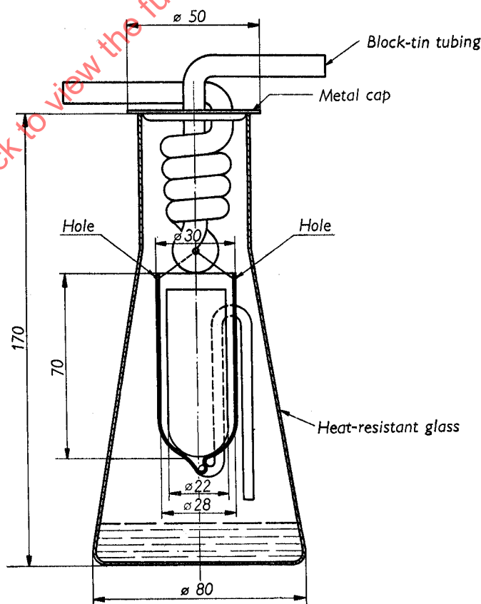
EXTRACTION APPARATUS
