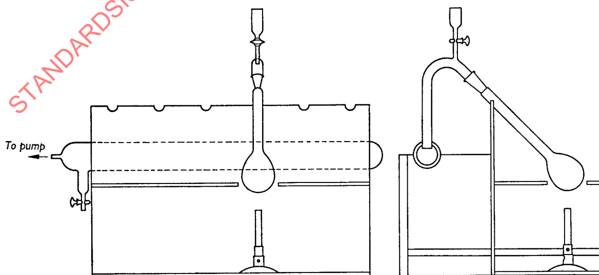
FIG. 1. — Wet oxidation apparatus
