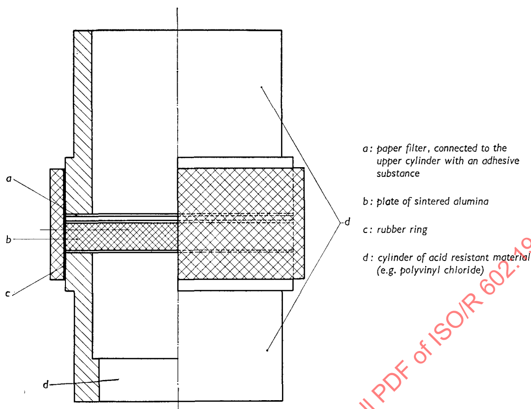
FIGURE. — Filtering device (Left half shown in section)
