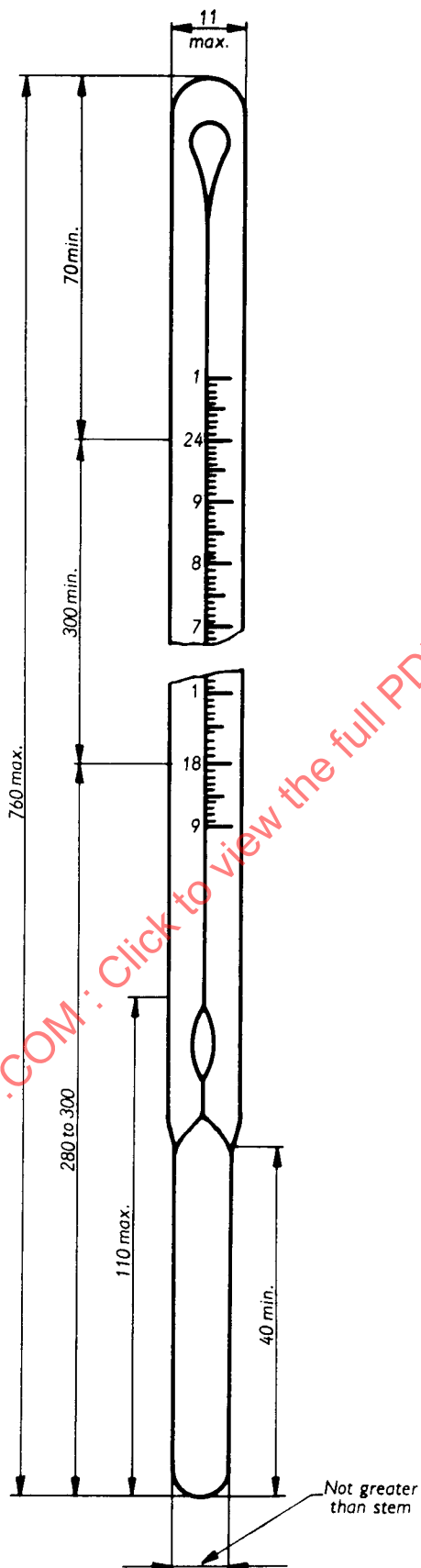
FIG. 1 — Solid-stem calorimeter thermometer Dimensions in millimetres
