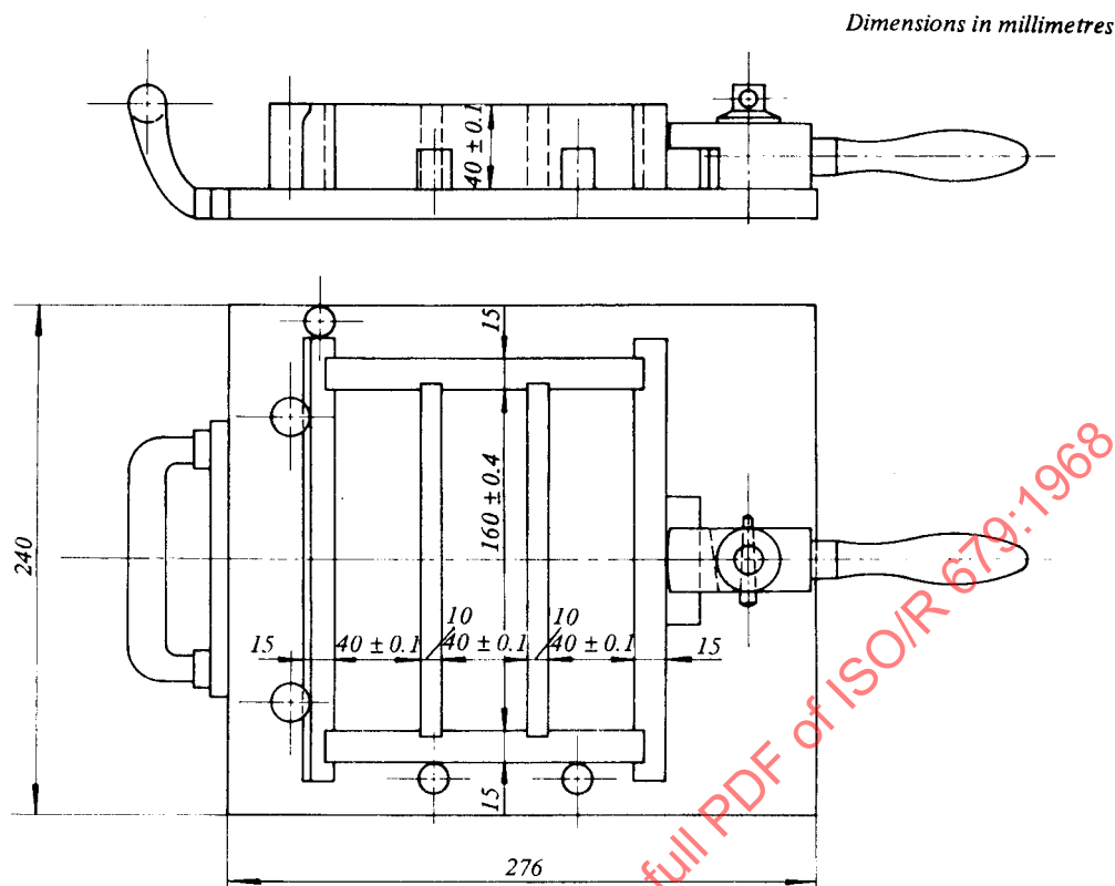
FIG. 3 – Type of mould for three prisms
