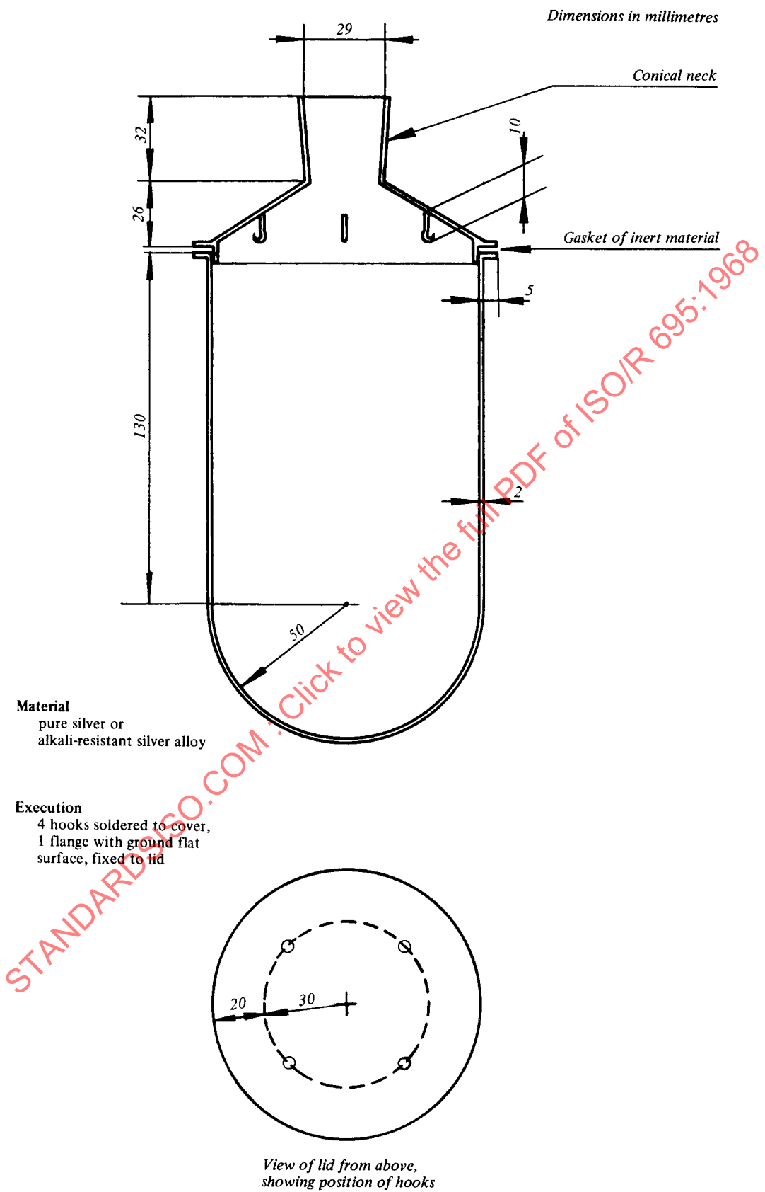
FIGURE – Example of suitable cylindrical silver vessel
