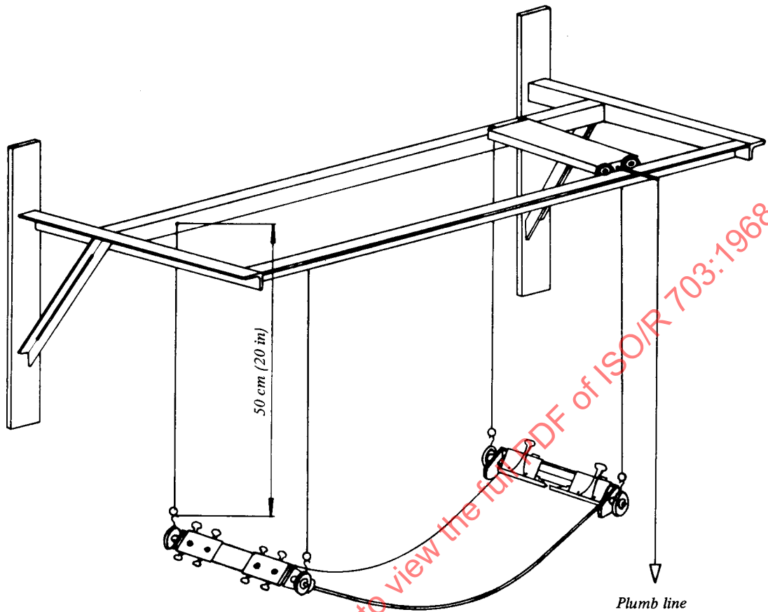
FIG. 1 – Apparatus for measuring deflection of test piece (Details given only as an indication)
