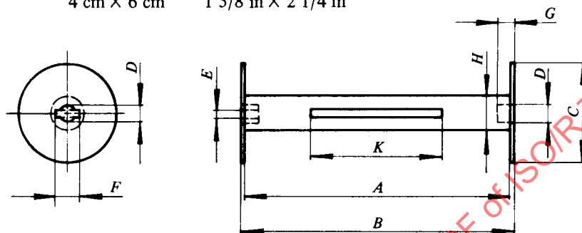
FIG. 6 – 620 roll film spool
