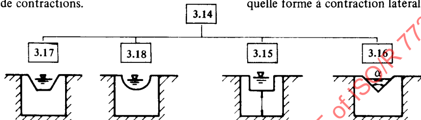
FIG. 20 – Notches
