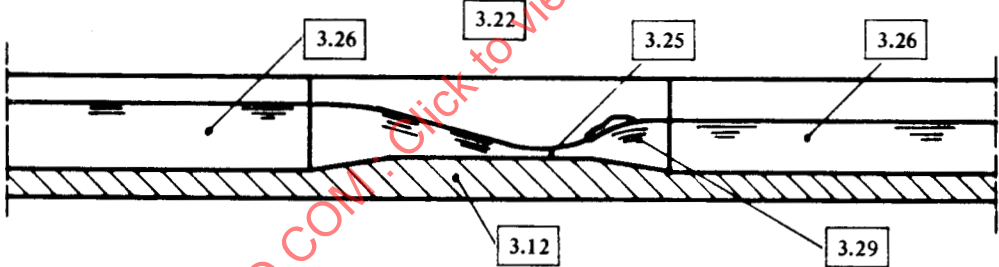
FIG. 23 – Standing-wave flume
