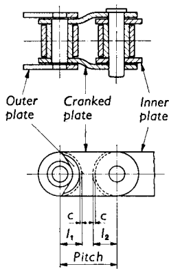
Cranked link
