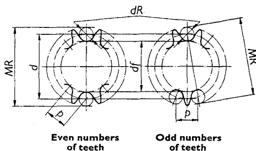
FIG. 4. — Diametral dimensions
