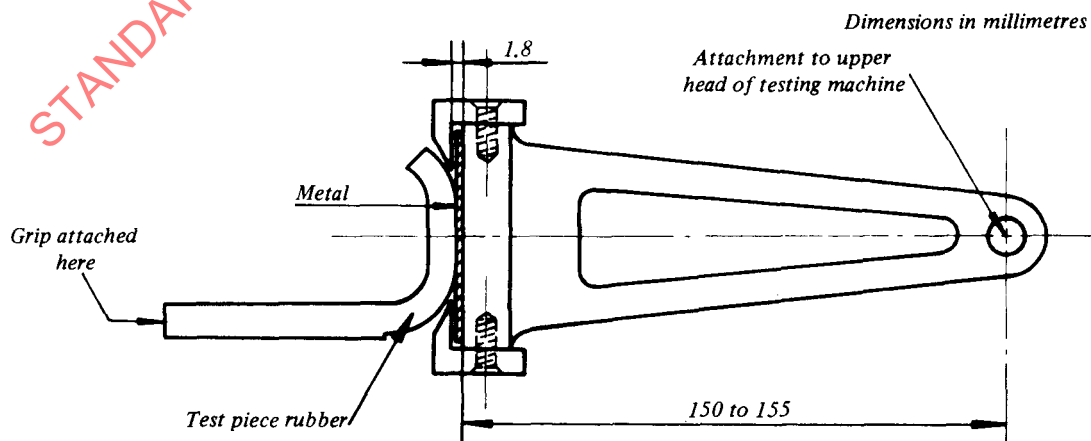
FIG. 1 — Test fixture for the adhesion test. The tensile force is applied at an angle of 90° to the plane of the rubber-to-metal bond.
