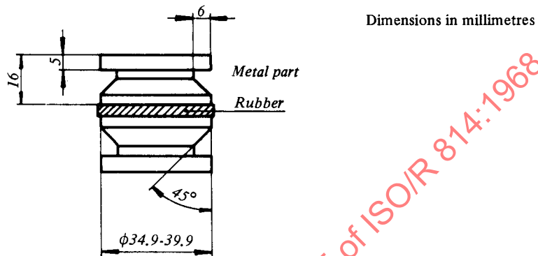
FIG. 2 — Example of standard test piece
