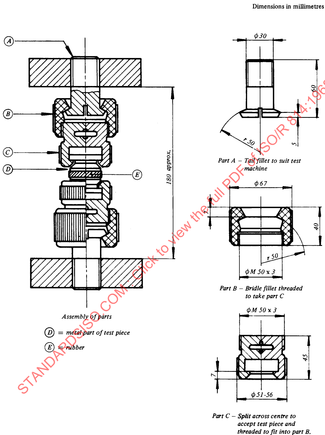
FIG. 1 – Test fixtures for holding rubber-to-metal bond test pieces
