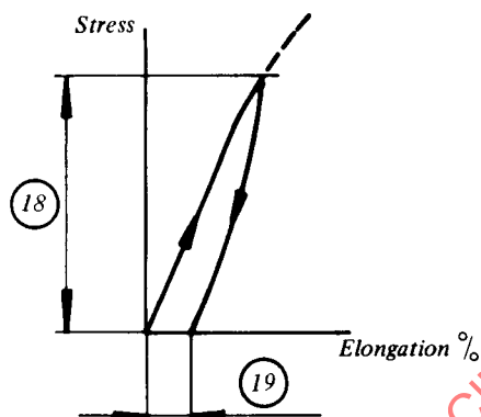
FIG. 4a – Determination of permanent set stress
