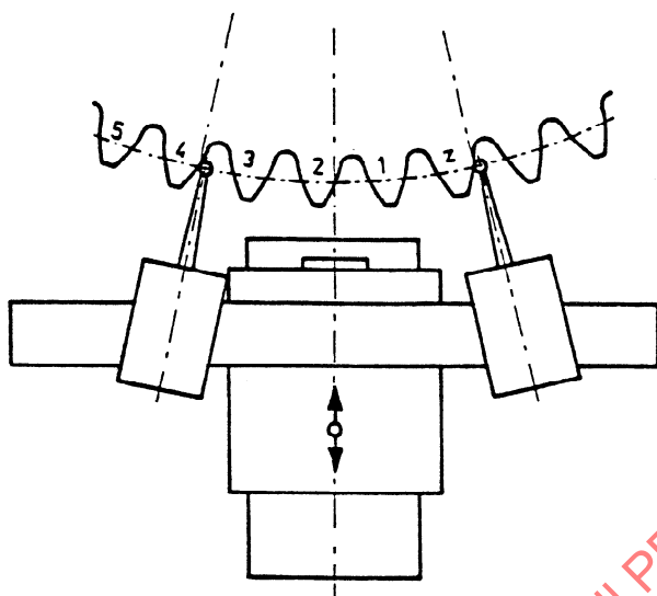
Fig. 13 Principle of pitch measurement by sectors
