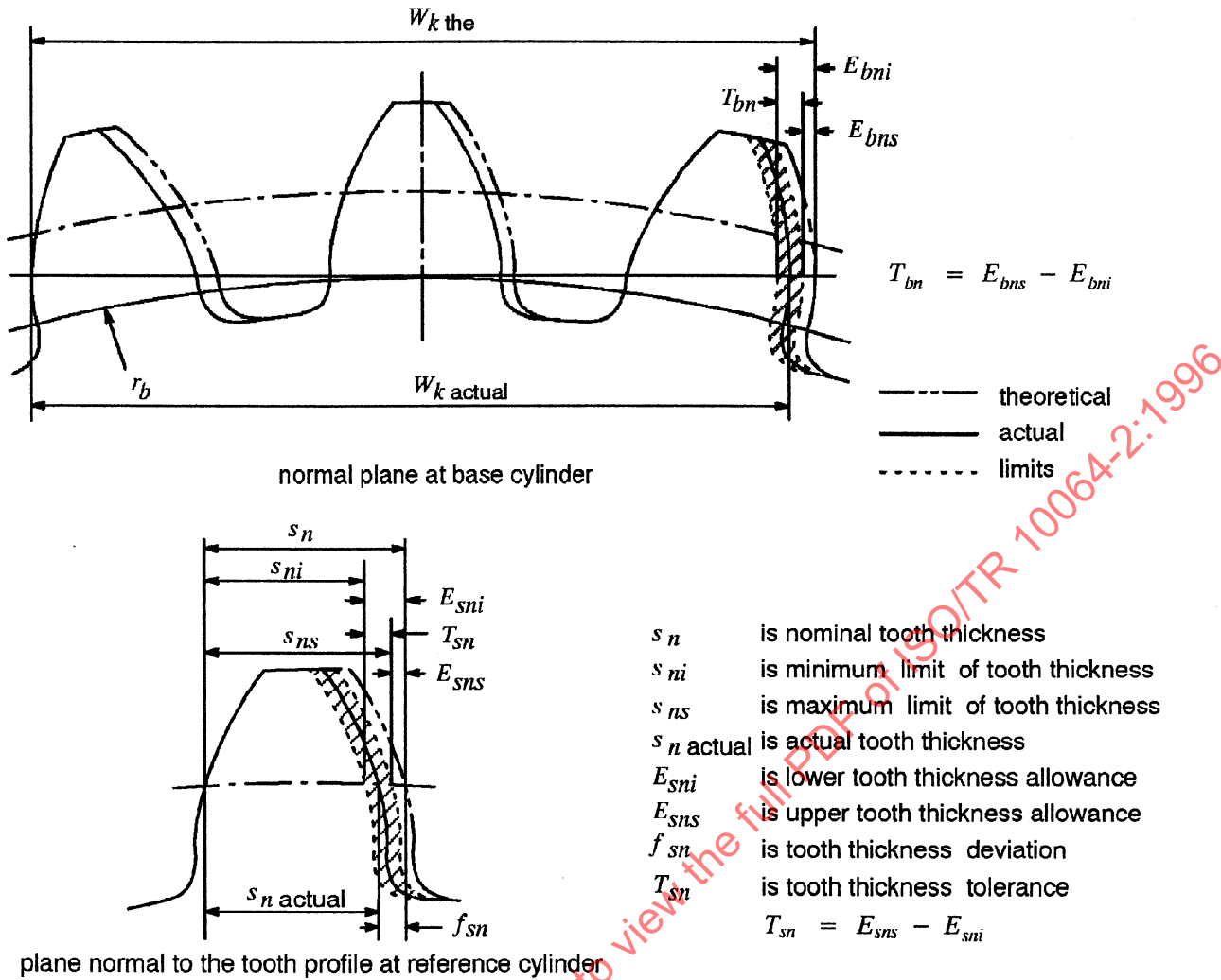
Figure 1 - Span and tooth thickness allowances
