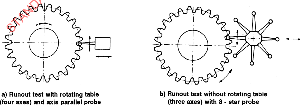
Figure 9 - Runout from coordinate measuring machine
