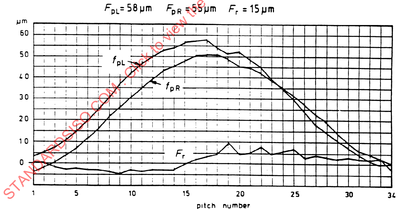
Figure 14 - Actual gear with little runout and substantial cumulative pitch deviation
