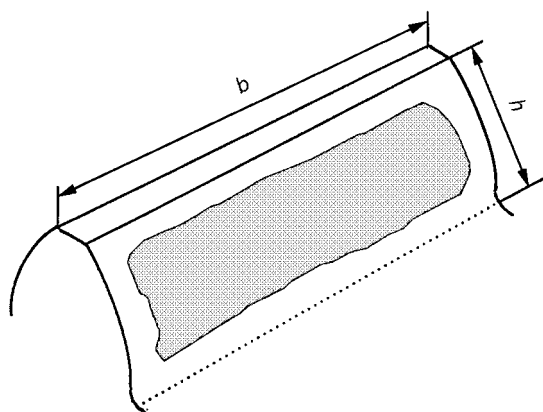
Figure 14 — Typical specification, contact approximately b = 80\% h = 70\% , tooth ends relieved
