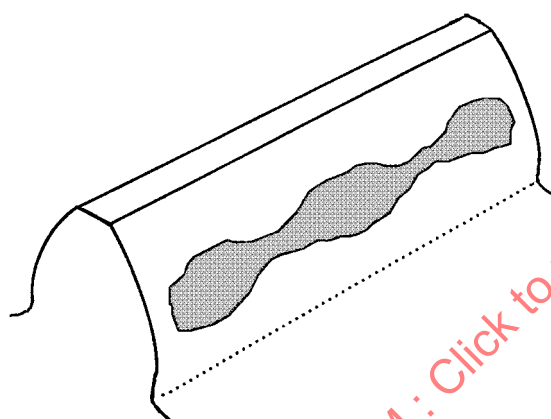
Figure 16 — Waviness
