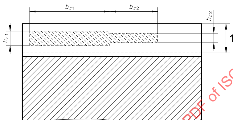
Figure 18 — Schematic distribution of contact pattern
