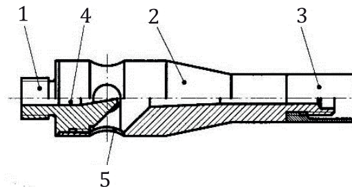
a) Burner assembly
