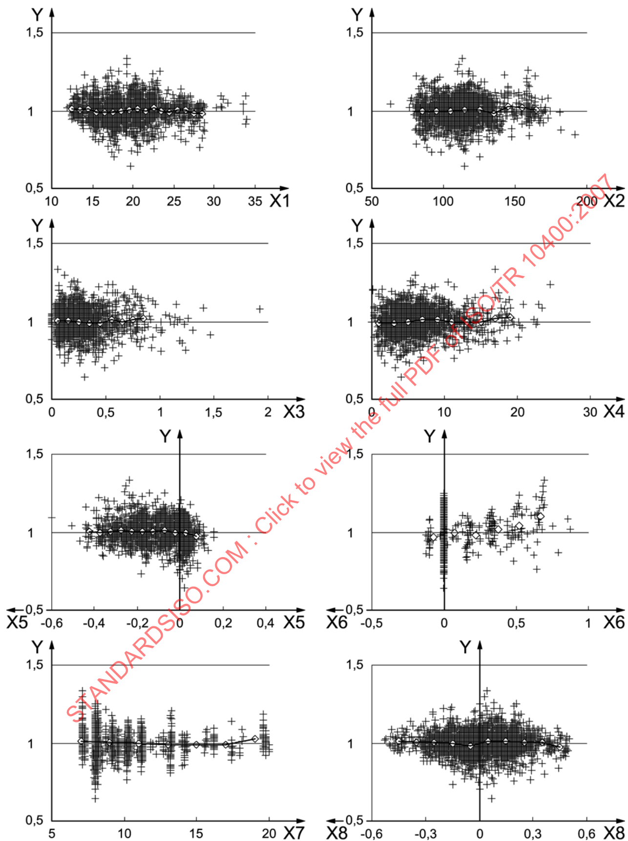
Figure F.2 (continued)
