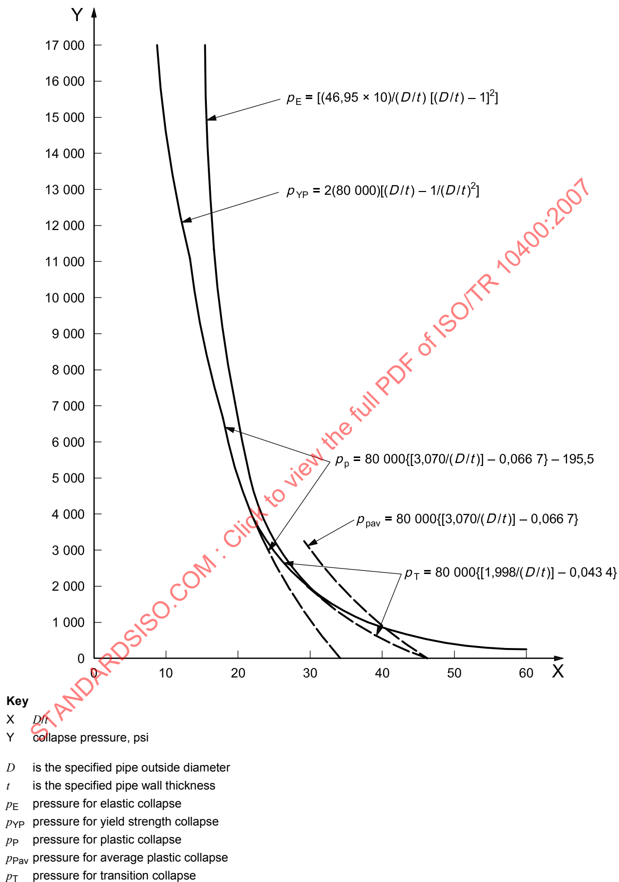
Figure E.1 — Grade N80 transition collapse equation derivation
