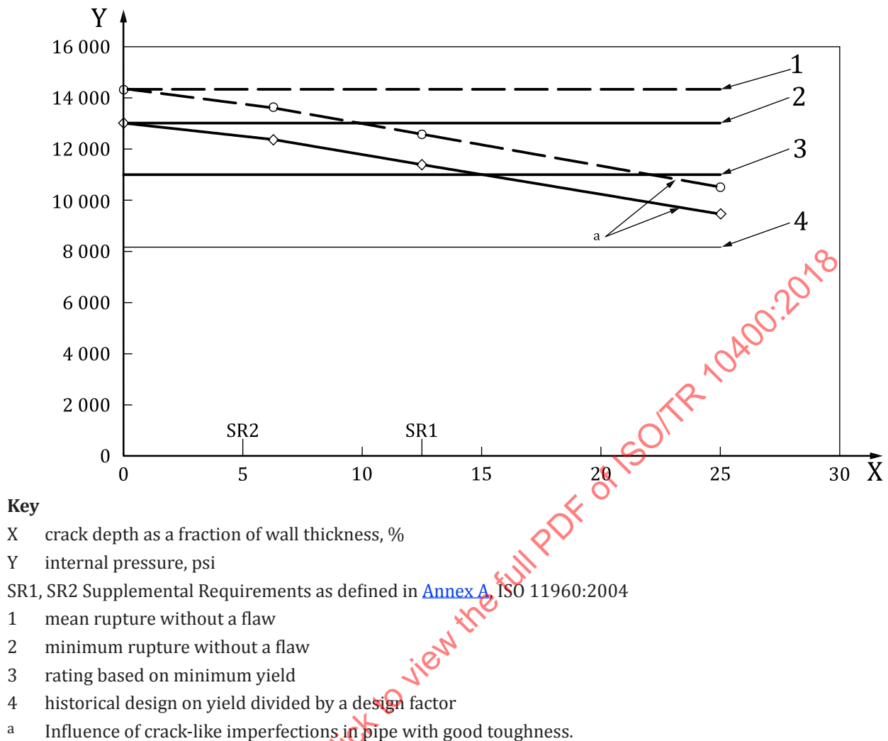
Figure B.5 — Influence of the imperfection penalty for 9-5/8 in, 53,5 lb/ft, P110 casing
