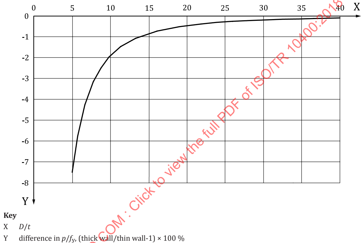
Figure A.4 — Comparison of thick and thin wall predictions of yield pressure for internal pressure only and zero axial load, k_{\text{wall}} = 0,875
