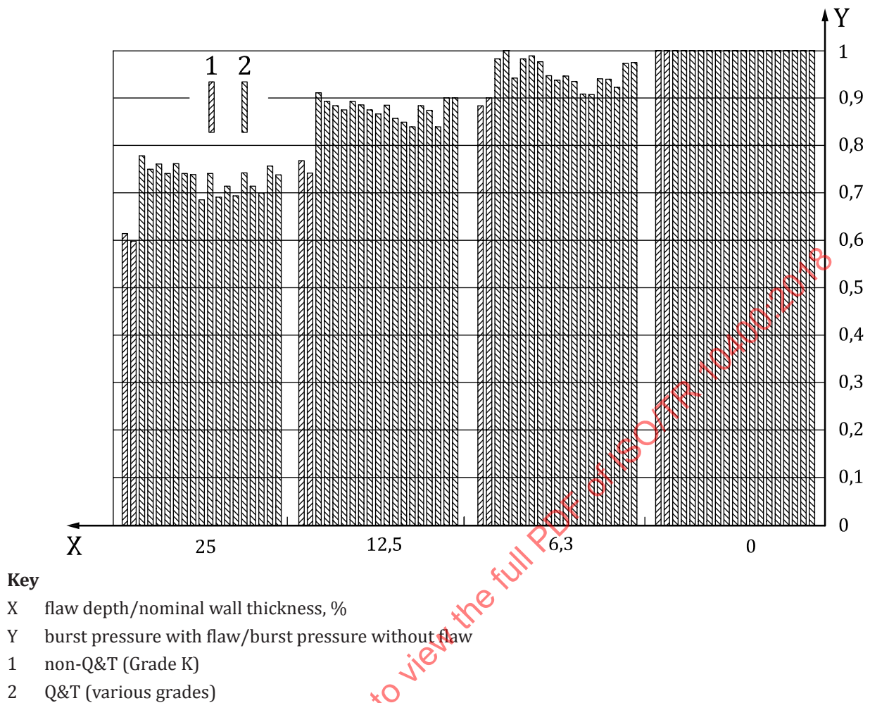
Figure B.8 — Influence of crack depth on ductile rupture
