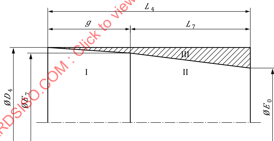
Figure 8 — Round threads and line pipe threads
