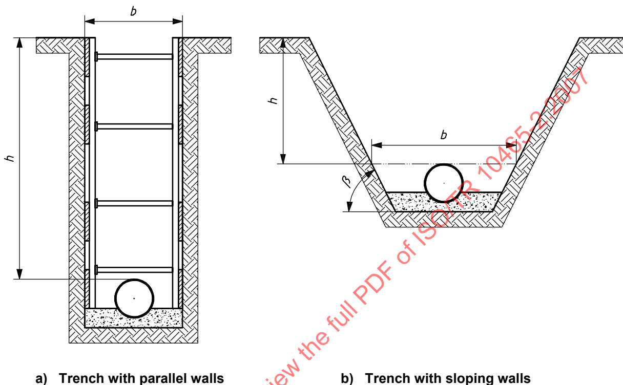
Figure 3 — Trench walls
