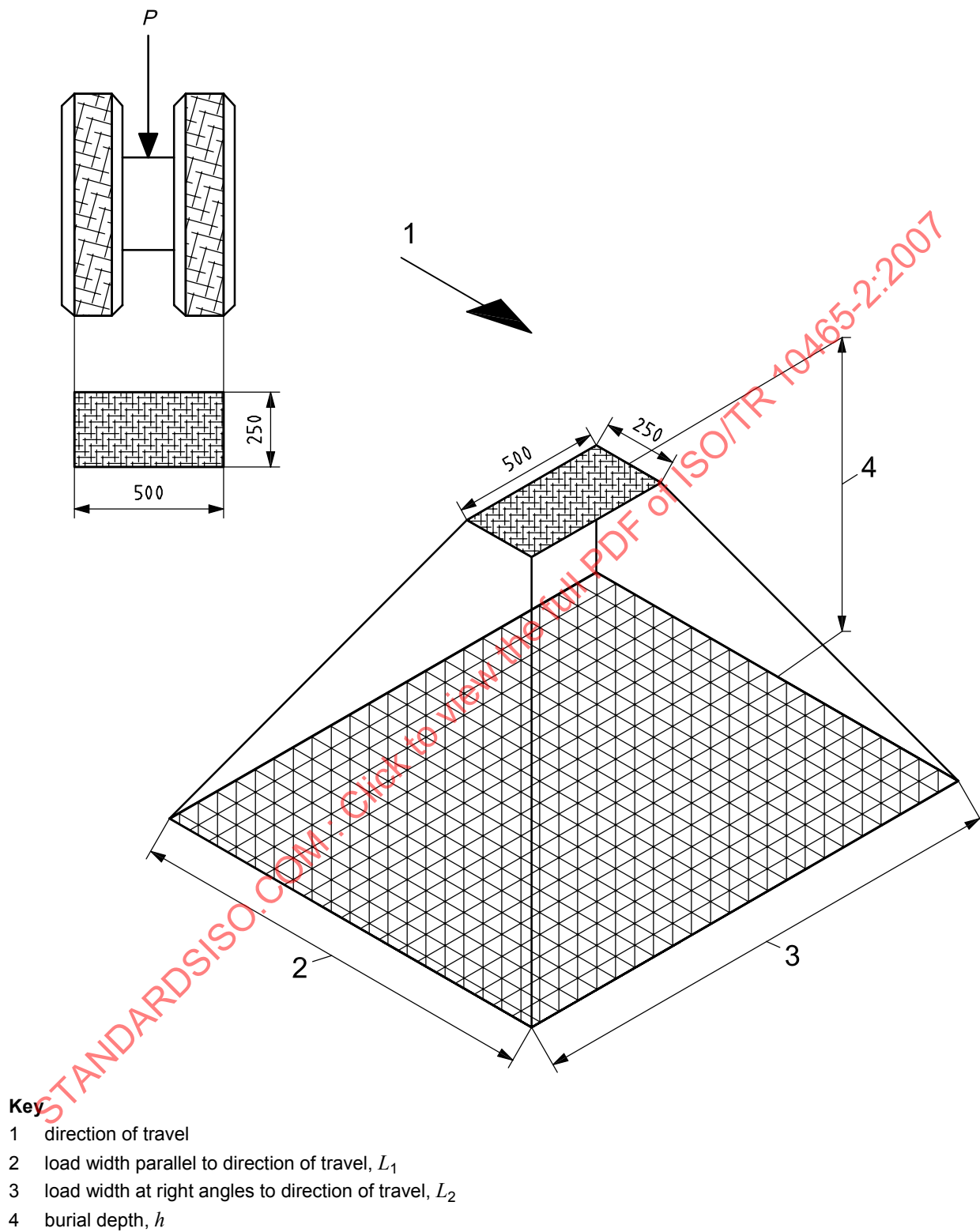
Figure 4 — Distribution of HS20 or HS25 live load through granular fill
