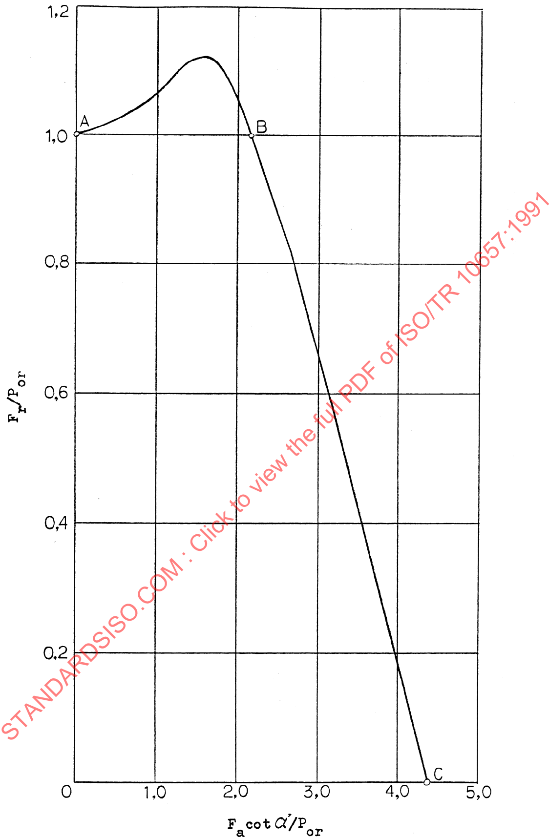
Figure 4-2 Theoretical relationship between radial and axial loads vs. static equivalent load for radial contact bearings
