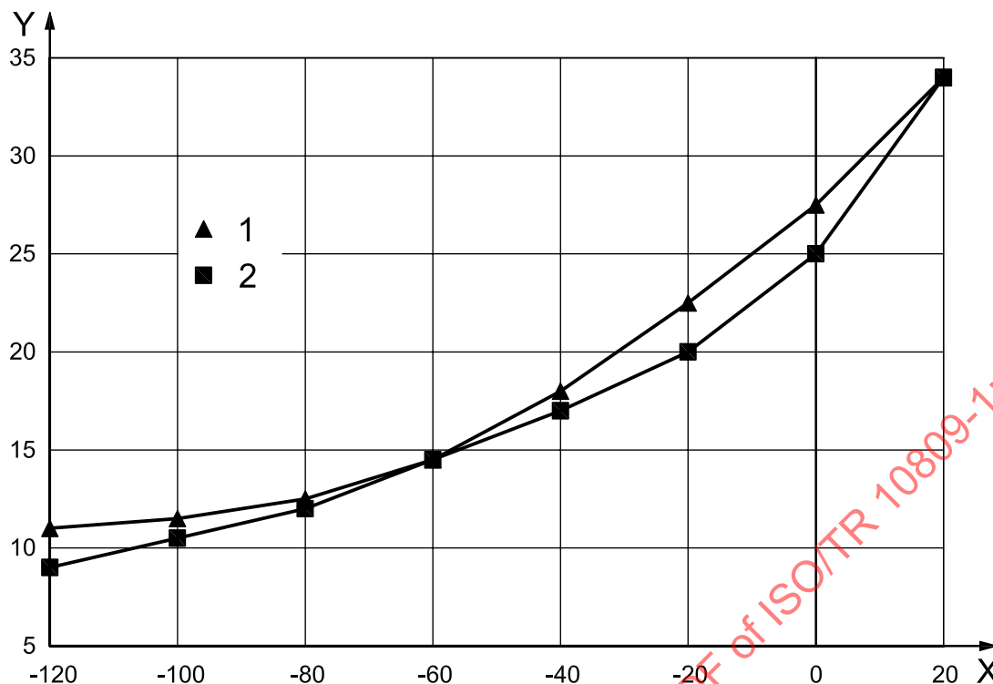
Figure 9 — Comparison of fracture toughness at various temperatures between ferritic ductile cast irons and low-carbon steels
