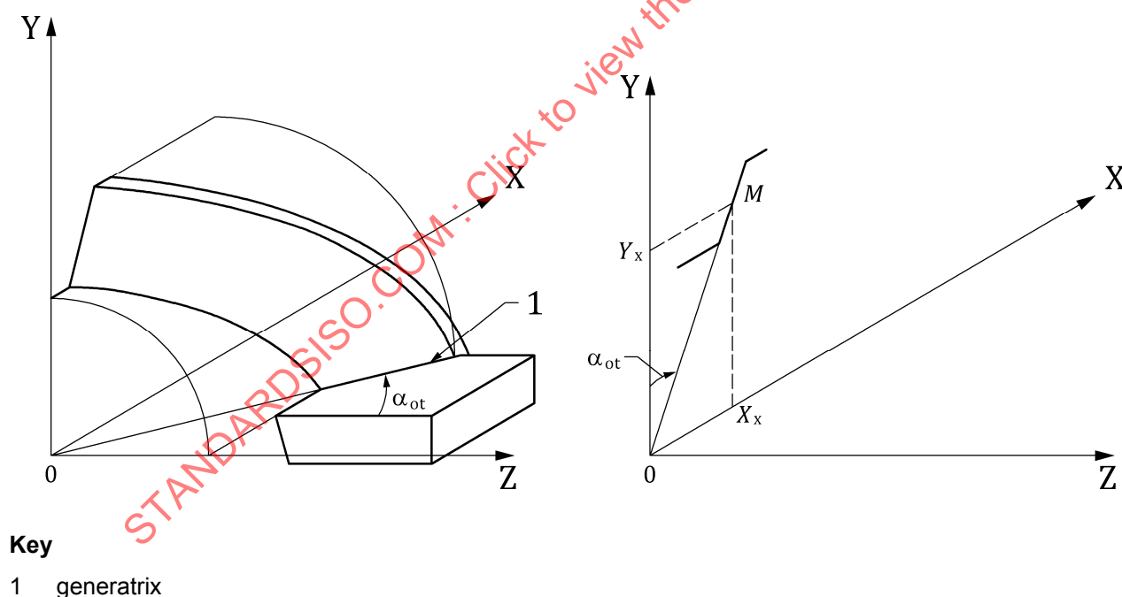
Figure A.1 — Generation of Type A profile
