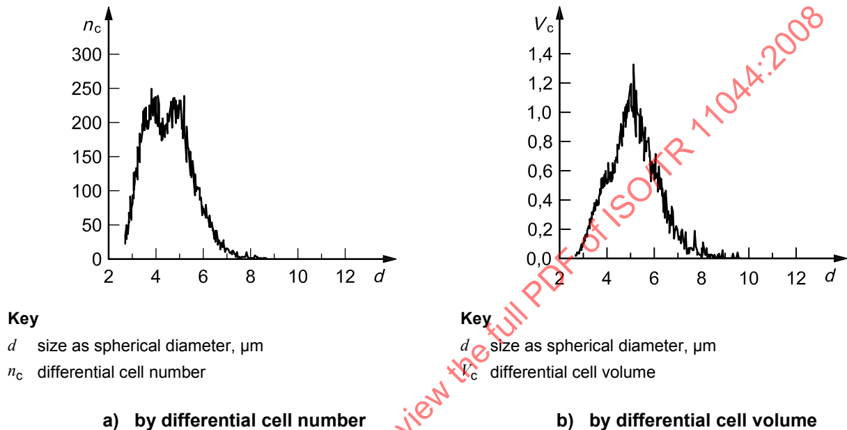
Figure 5 — Size distributions of a culture of P. subcapitata in the exponential growth phase in ISO 8692 growth medium
