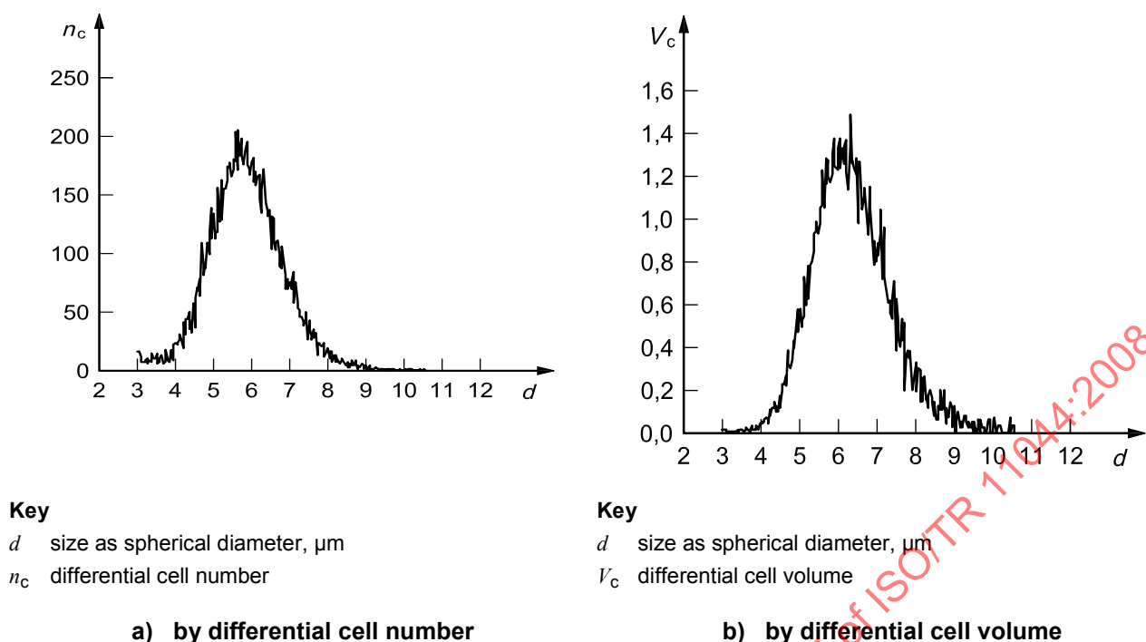
Figure 8 — Size distributions of a culture of S. costatum strain NIVA BAC 1 ( S. pseudocostatum ) in the exponential growth phase in ISO 10253 growth medium based on natural sea water
