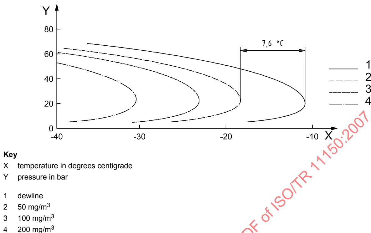
Figure 4 — Gas 3 condensation behaviour
