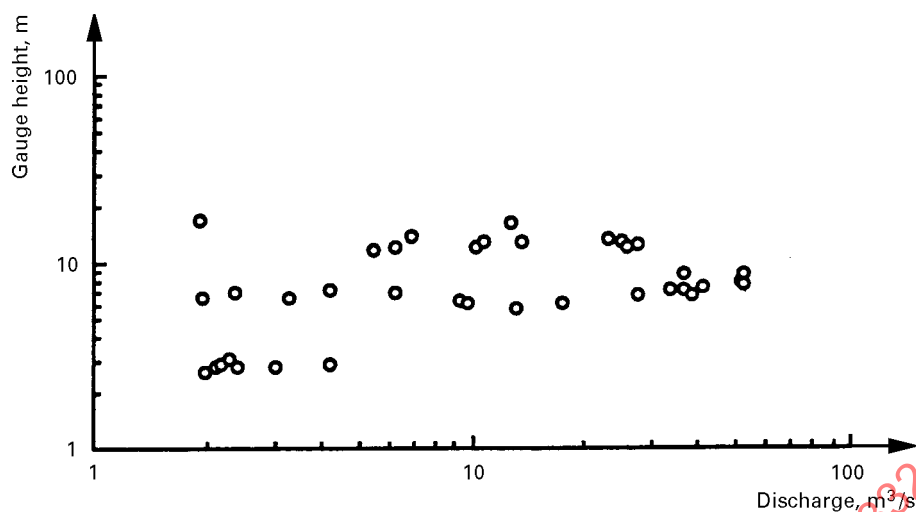
a) Discontinuous stage-discharge relation
