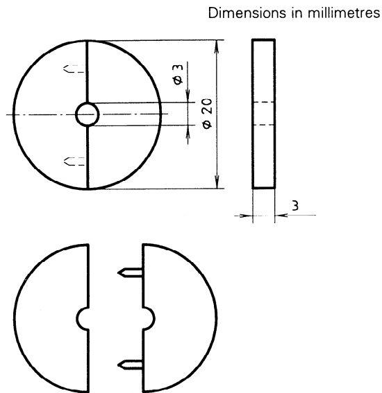
Figure 8 — Split mould
