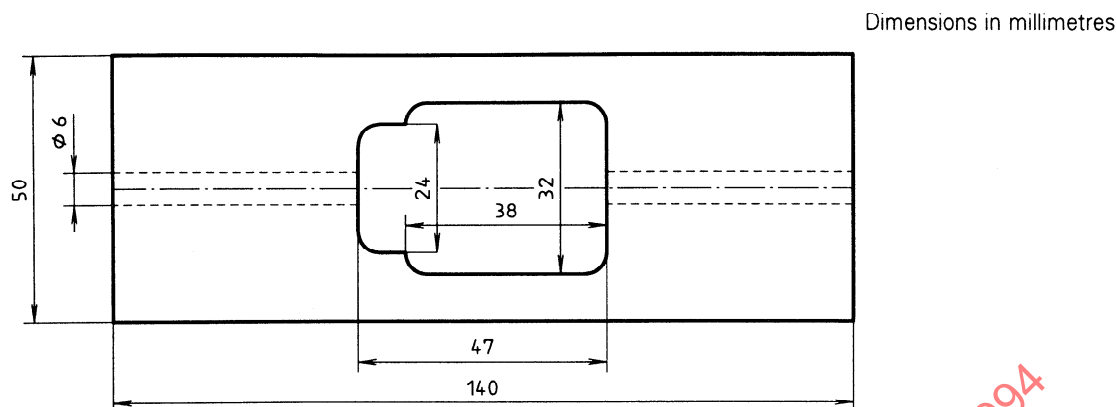
Figure 5 — Alternative measurement alignment block
