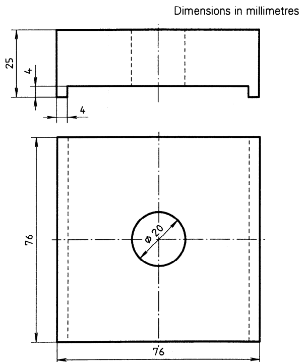
Figure 4 — Polishing block
