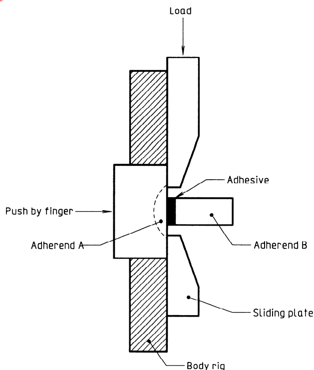
Figure 6 — Schematic diagram of testing jig for shear bond strength
