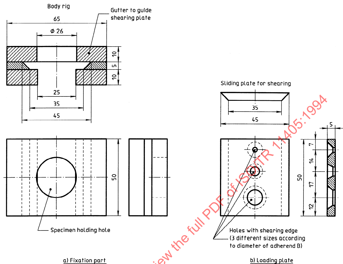
Figure 7 — Constructional figure of rig for bond strength measuring by shear
