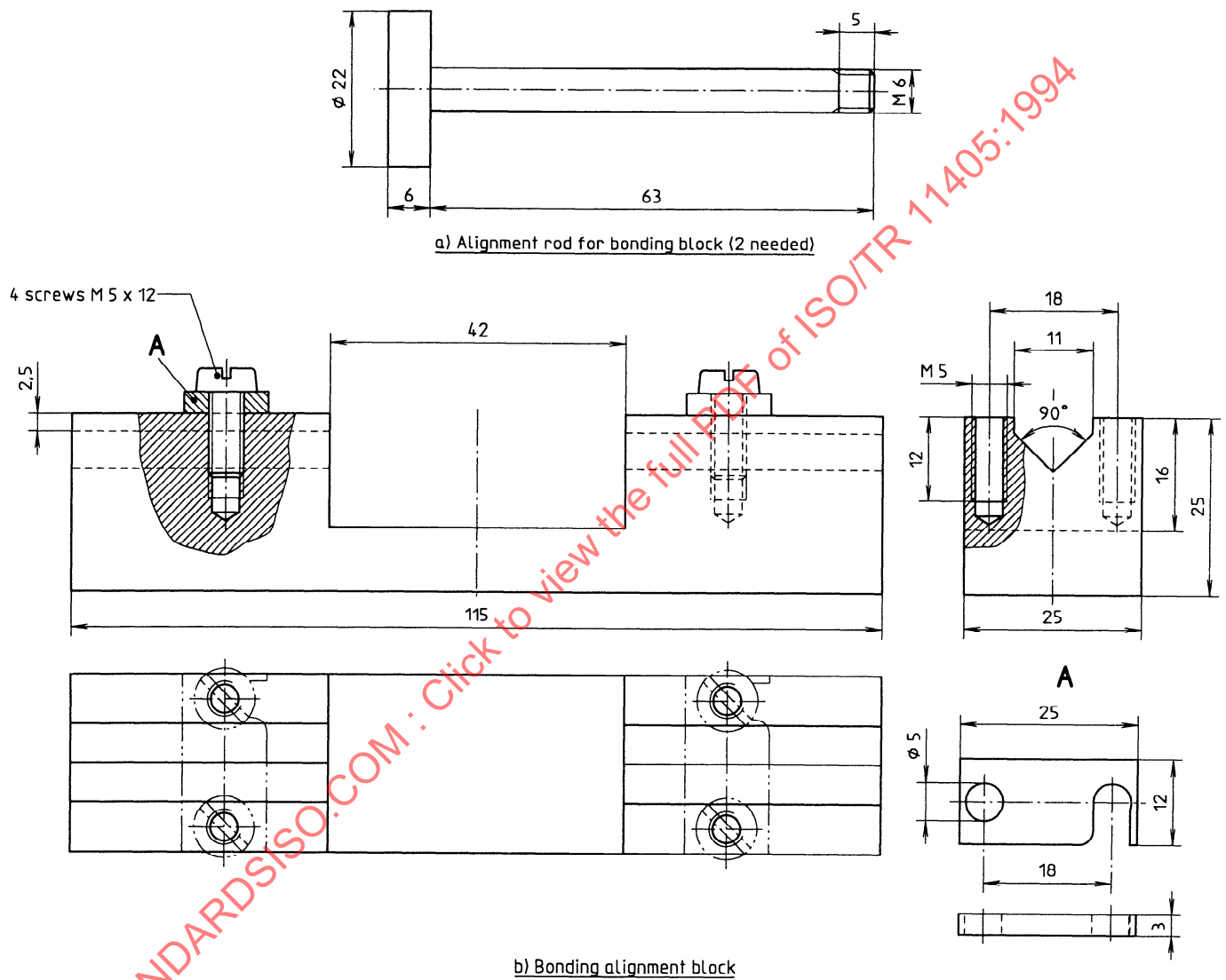
Figure 2 — Bonding alignment apparatus
