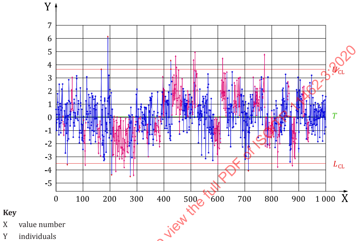
Figure 28 — Individuals control chart for test data set 4
