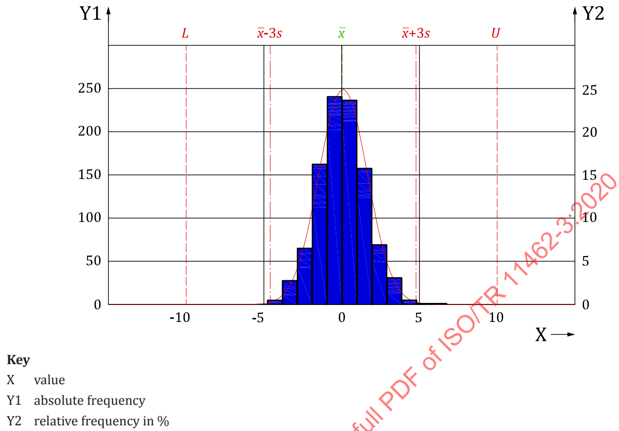
Figure 25 — Histogram of test data set 4
