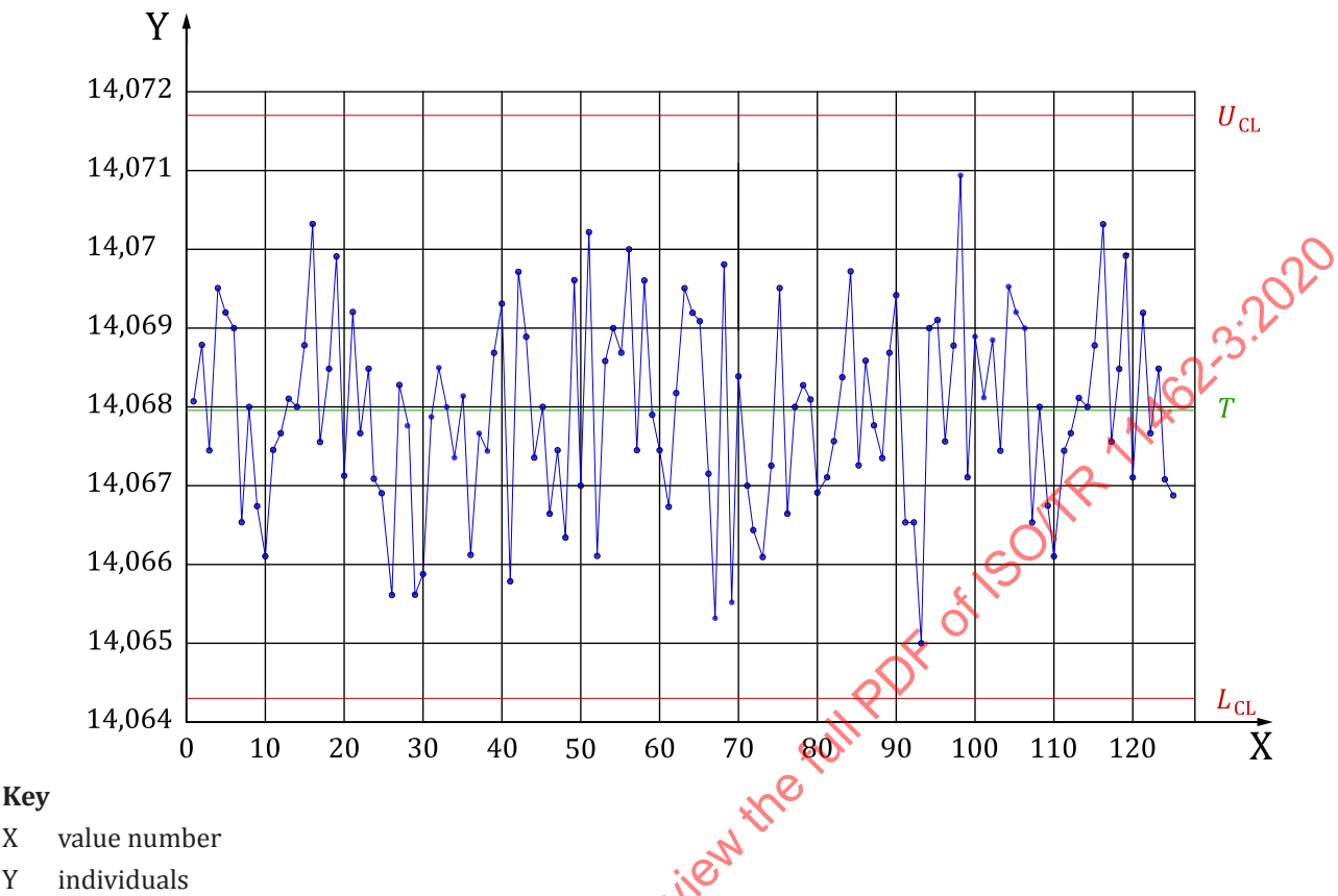
Figure 4 — Individuals control chart for test data set 1
