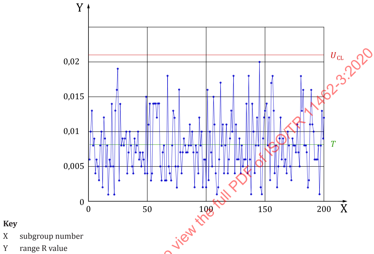
Figure 15 — R control chart for test data set 2
