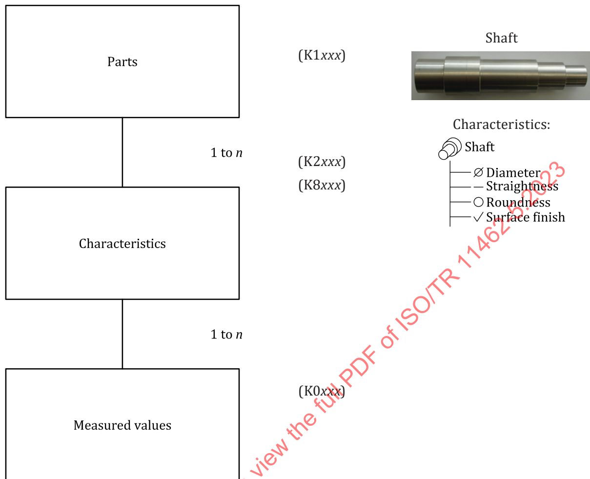
Figure 1 — Data model
