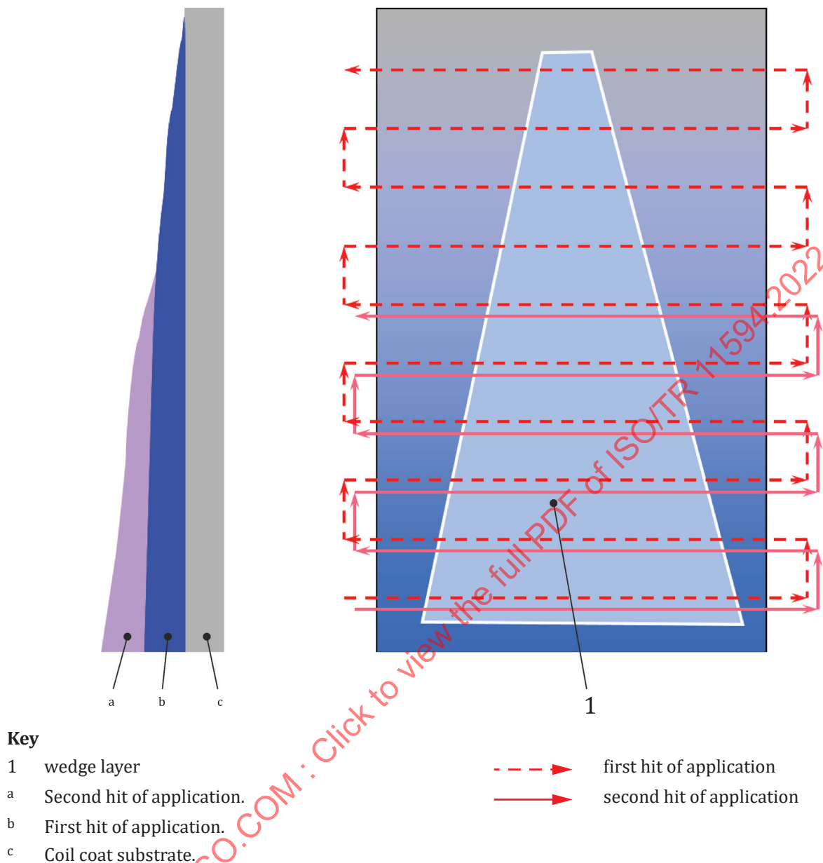
Figure 2 — Creation of a wedge-shaped layer
