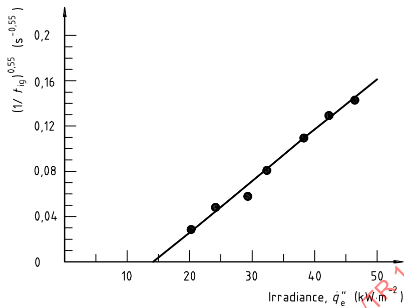
Figure A.1 — Correlation of ignition data for a cellulosic flooring material
