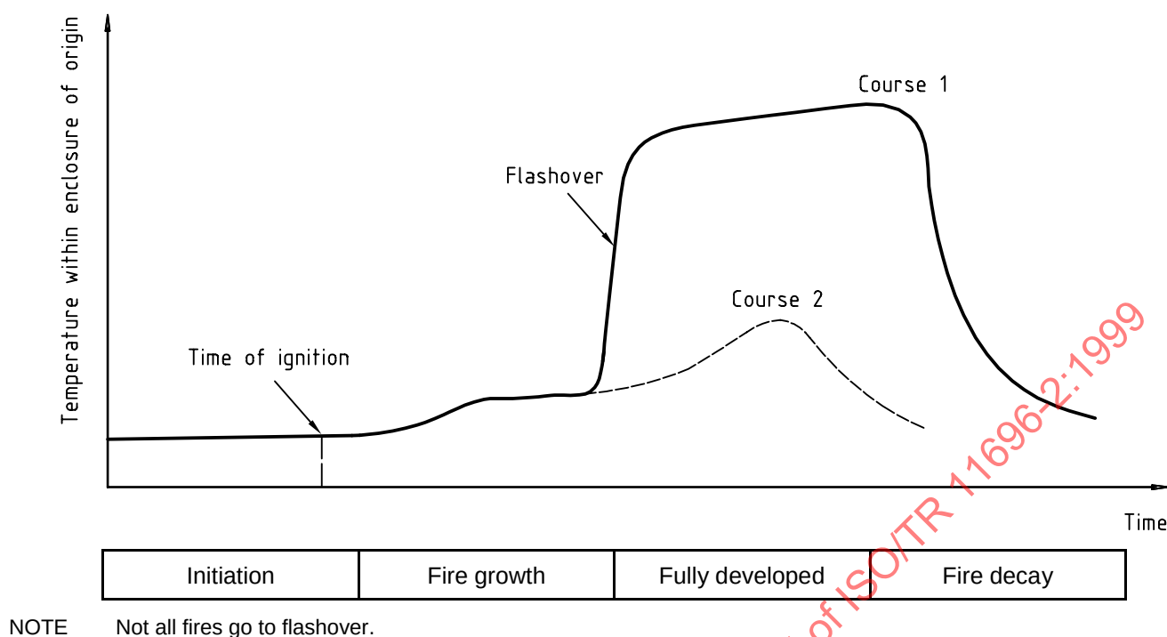
Figure 1 — Diagram showing the different phases in the development of a fire within an enclosed space
