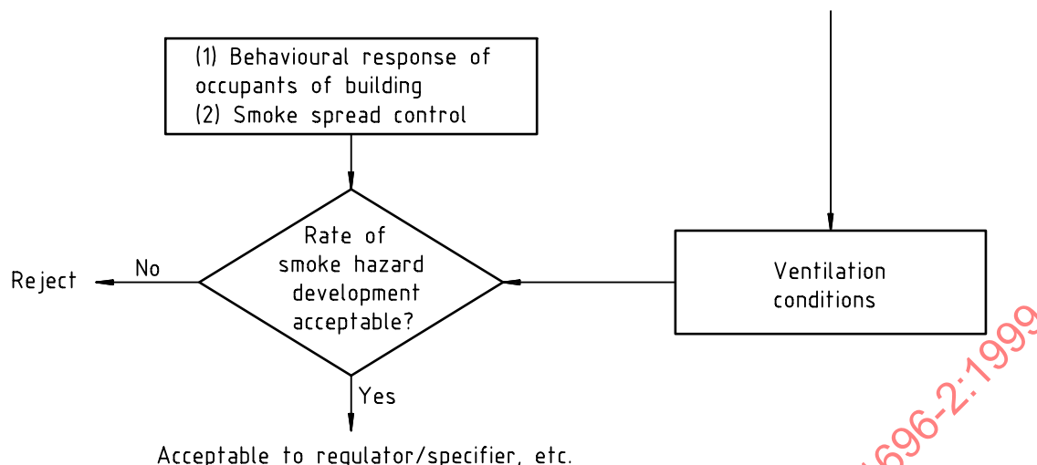
Figure 8 — Fire hazard assessment: Step 5
