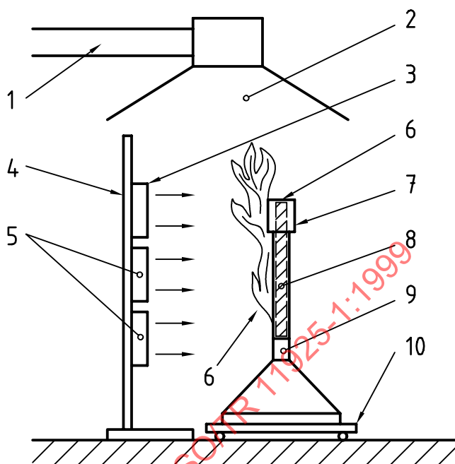
Figure 5 a) — Intermediate-scale calorimeter
