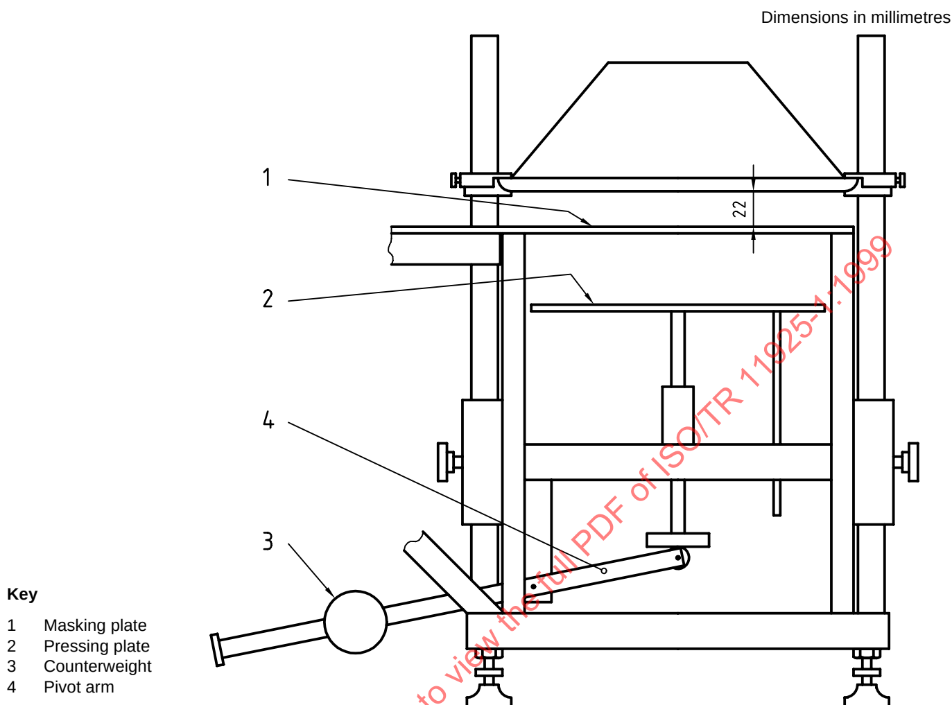
Figure 1 a) — Specimen support framework and radiator cone
