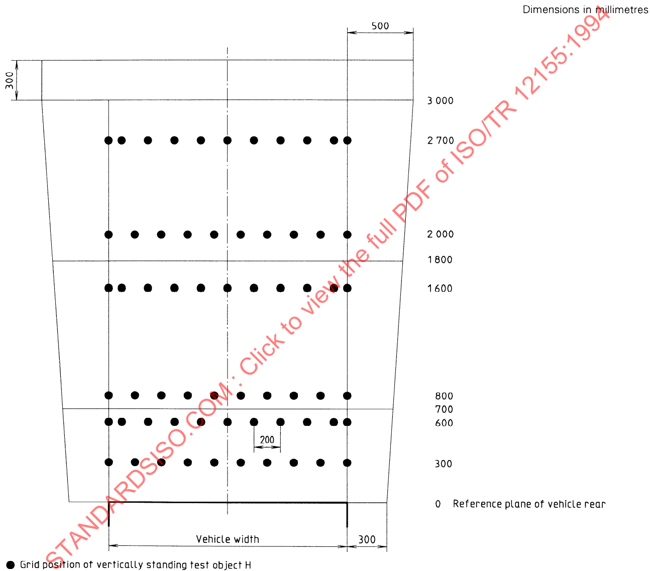
Figure 3 — Test 1 (plan view)
