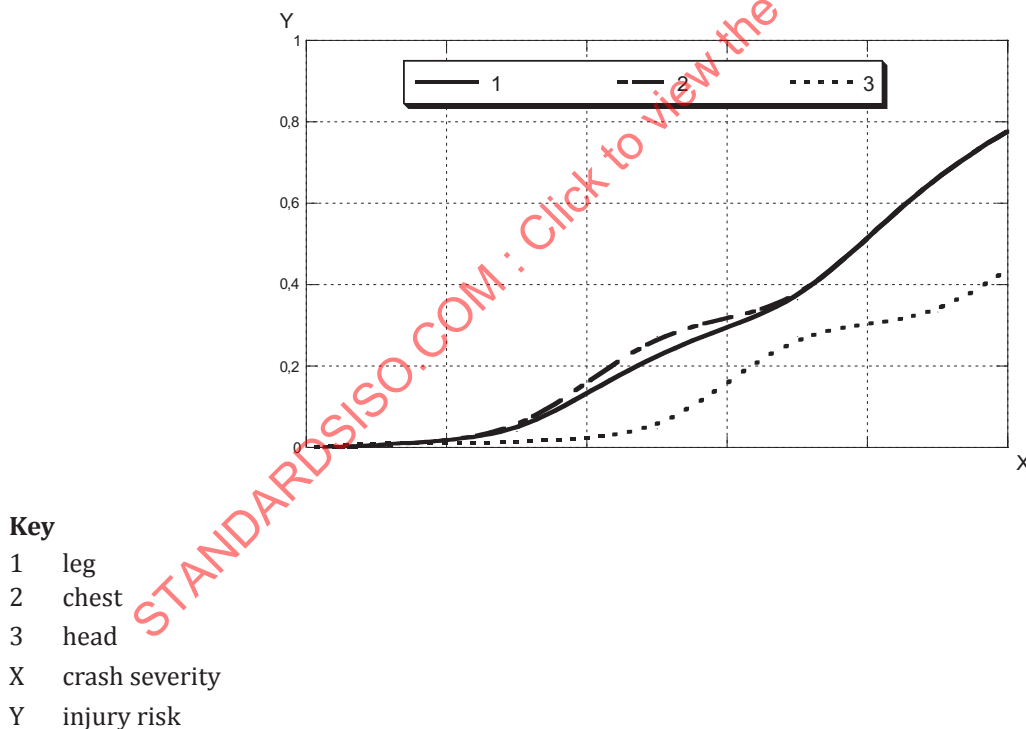
Figure B.1 — Reported AIS 2+ rate by body region versus \Delta v from crash pulse recorder data
