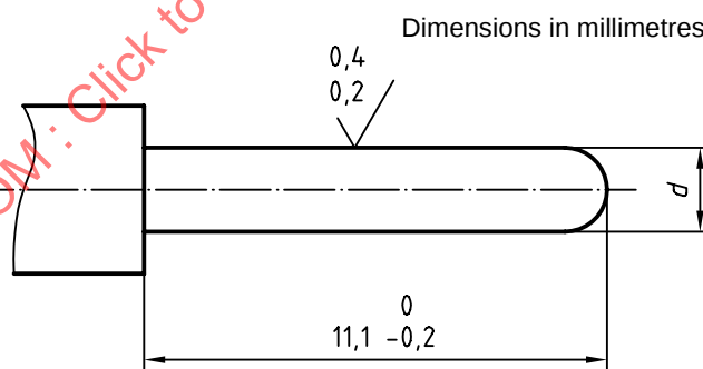
Figure 4 — Test pin
