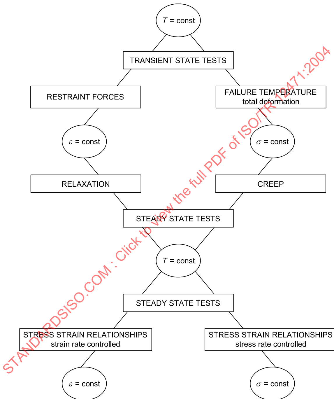
Figure 20 — Different testing regimes for determining mechanical properties of materials at elevated temperatures
