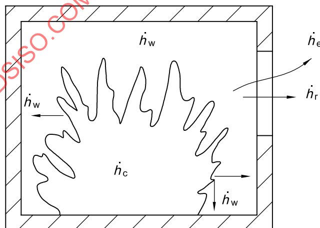
Figure 11 — Energy balance of a compartment fire
