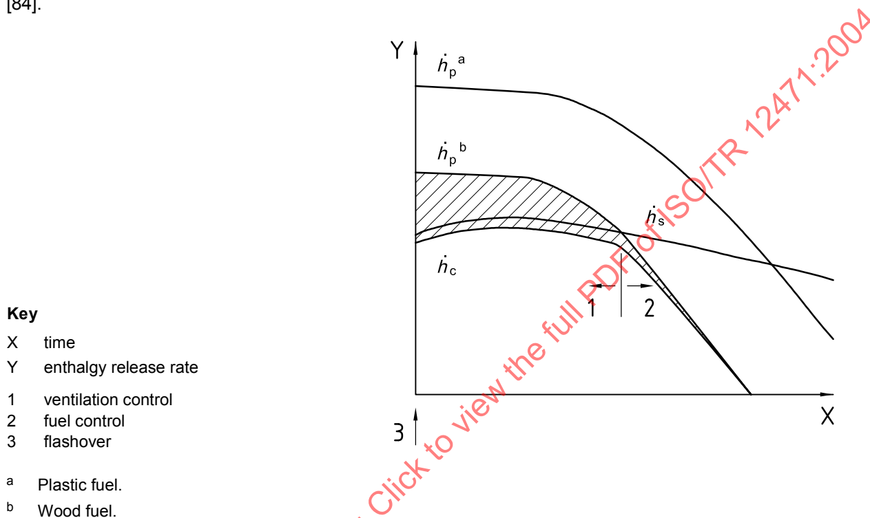
Figure 12 — Possible rates of enthalpy release in a fully developed compartment fire versus time for two types of fuel
