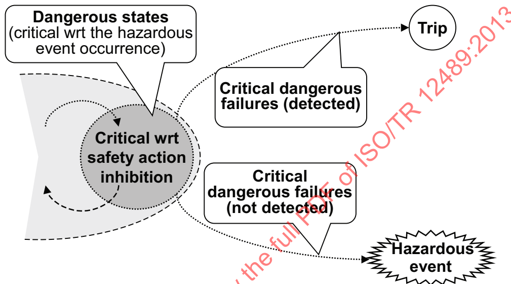
Figure B.4 — Equivalent representation of the states in left hand side of Figure B.3
