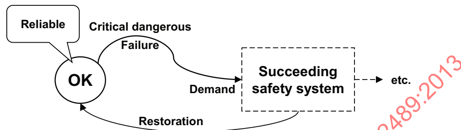
Figure 13 — Broad model for non-ultimate-continuous mode safety system
