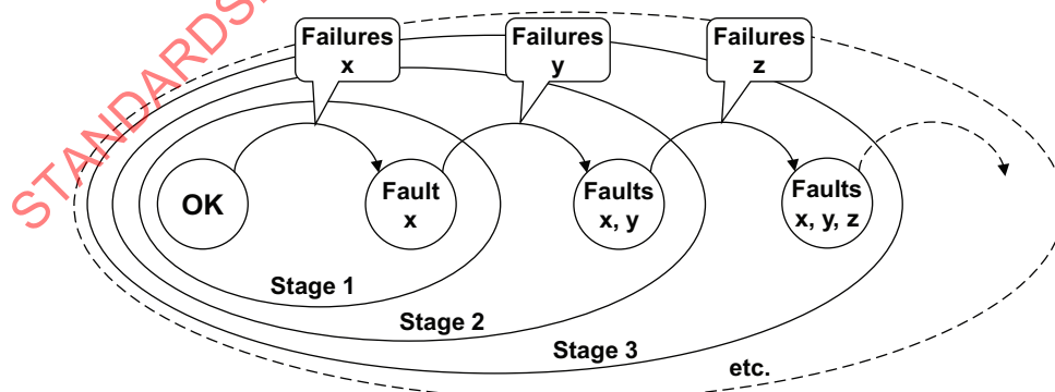
Figure 8 — Relationship between failure and fault concepts
