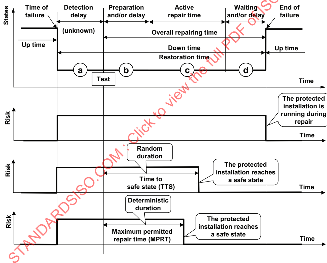
Figure 7 — Illustration of the restoration time and of the risk exposure for the hidden failures of an item
