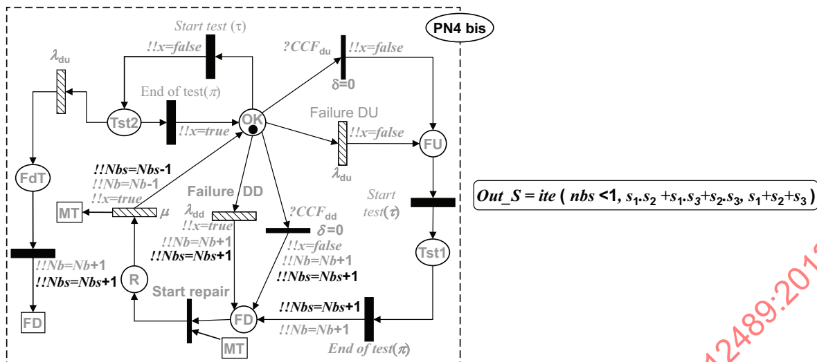
Figure 89 — Module PN4-bis and assertion to switch from 2003 to 1002
