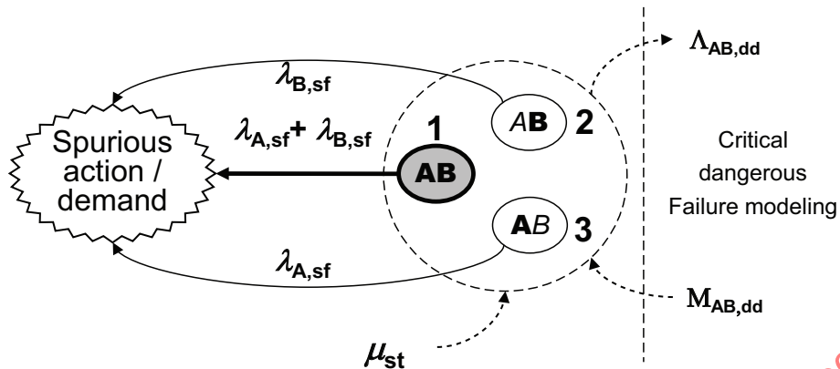
Figure I.11 — Spurious failure model - case 1002 -
