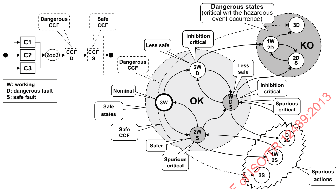
Figure B.2 — Example of the classes of states for a 2oo3 system
