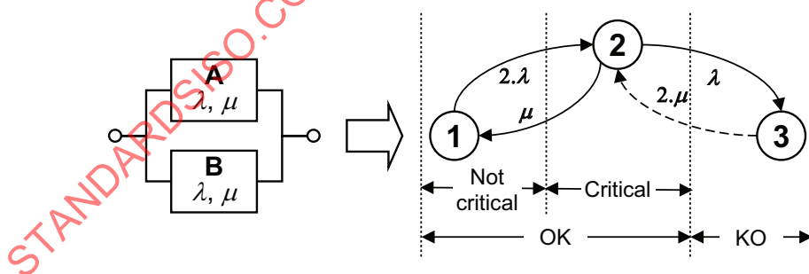
Figure C.5 — Simple system with two identical repairable components
