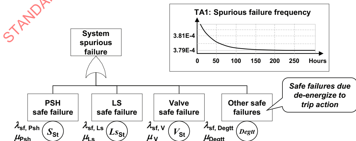
Figure 52 — TA1-1 Spurious failure frequency \Phi_{st}(t) as function of the time
