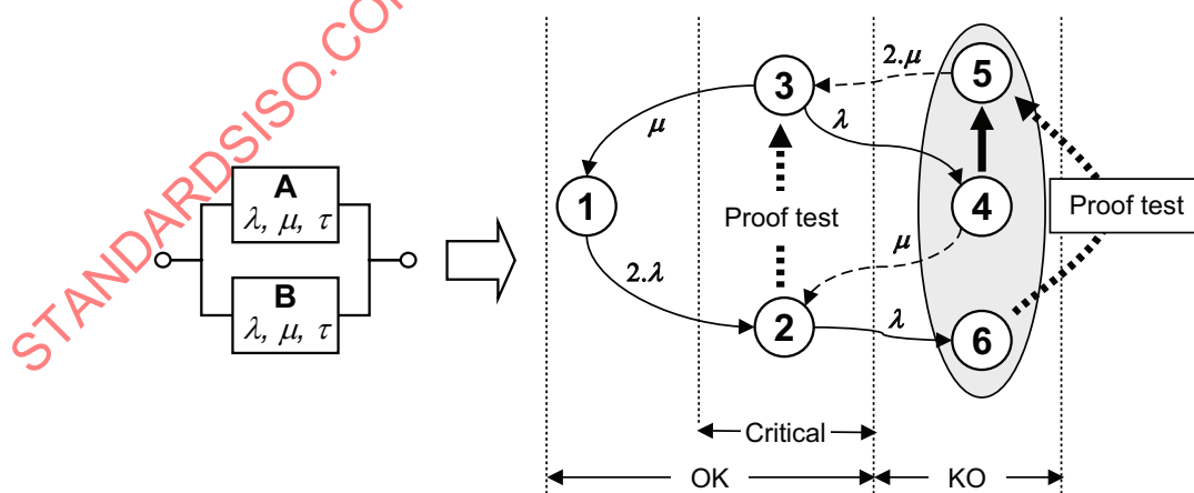
Figure C.10 — Simple system with periodically tested components
