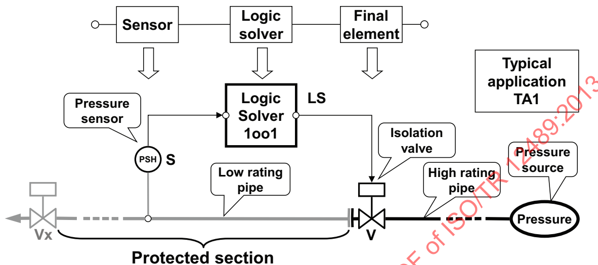
Figure 45 — Simplest basic architecture - Typical application TA1-1
