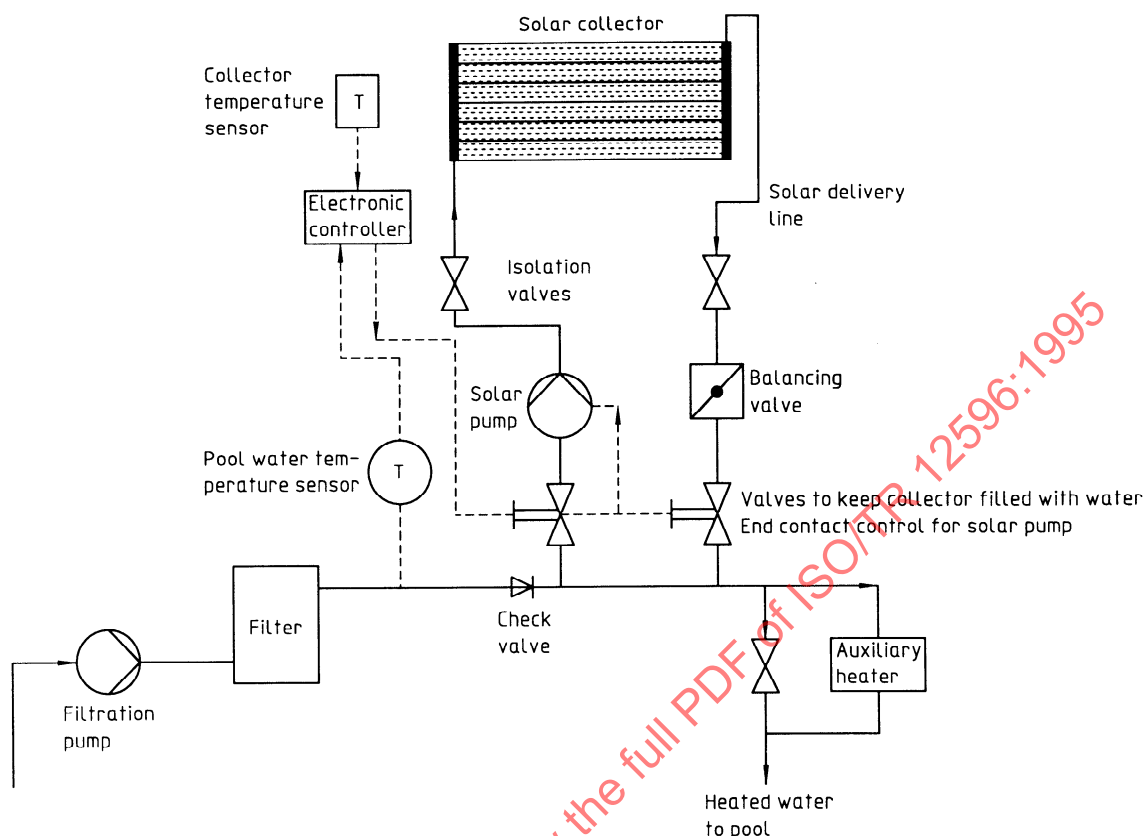
Figure 10 — Use of separate pump and hydraulic system applicable to large systems (more than 100 m 2 collector area)
