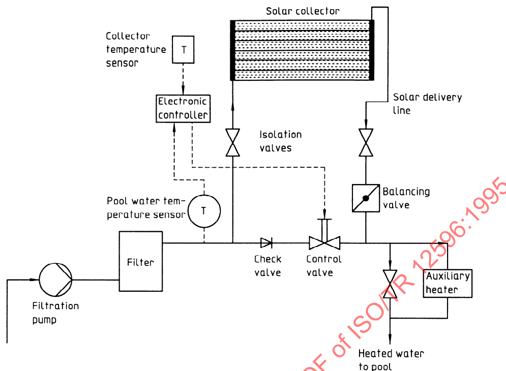
Figure 7 — Use of existing pump, single-valve arrangement
