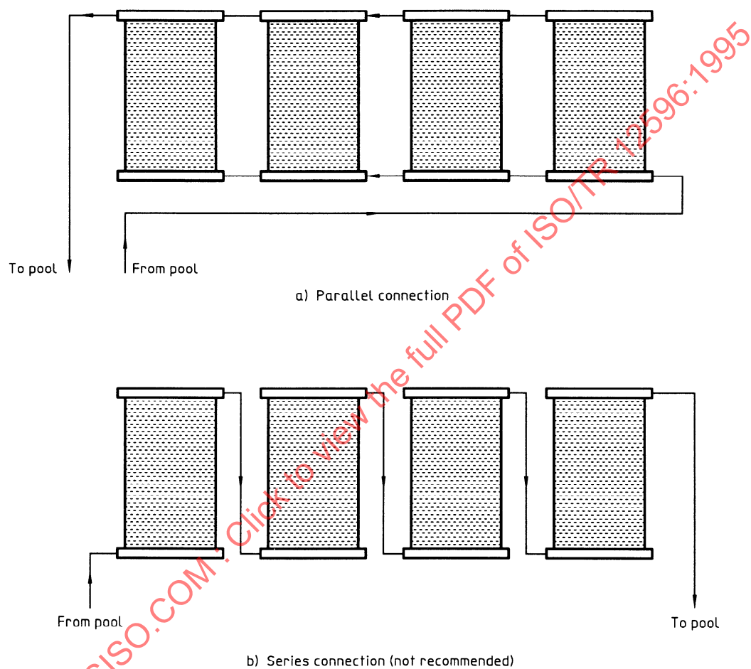
Figure 4 — Parallel and series connection of panel collectors
