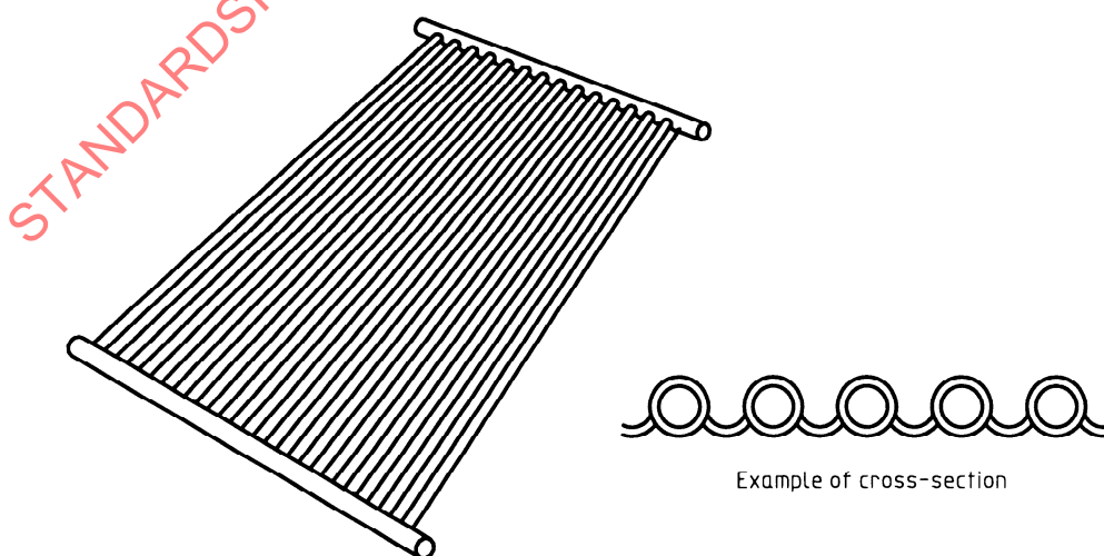
Figure 1 — Example of a plastic/elastomeric panel collector
