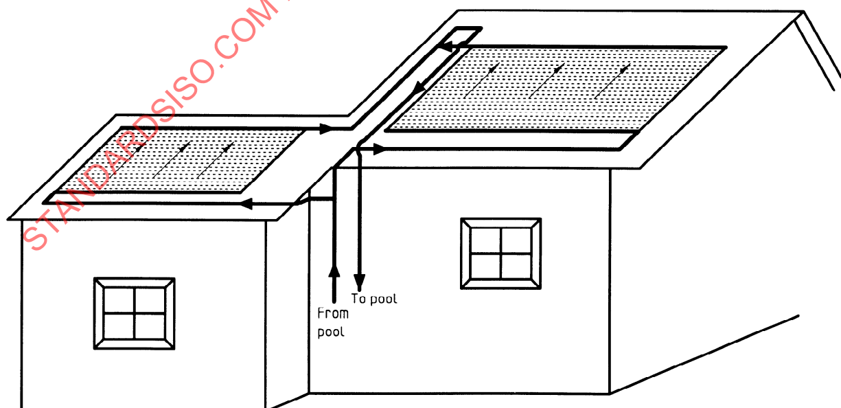
Figure 6 — Recommended plumbing arrangements for collector panels at different elevations
