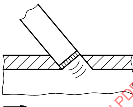
b) Transducer in contact with the fluid (flush)
