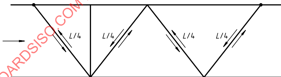
c) Indirect transmission (reflected by the conduit wall) (W-path)
