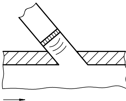
a) Transducer in contact with the fluid (retracted)
