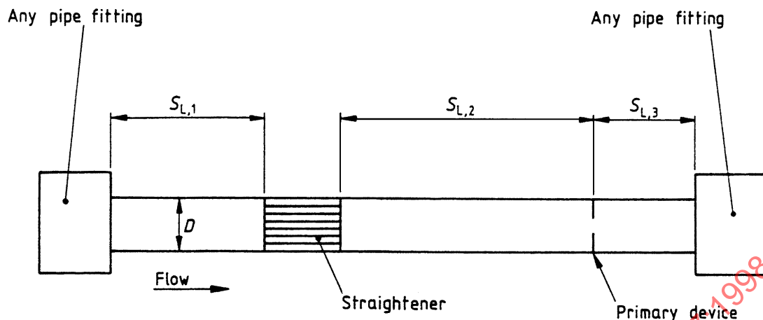
Figure 9 — Flow straightener installation
