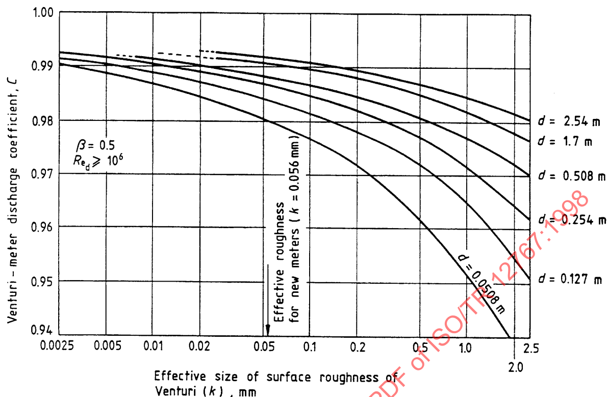
Figure 13 — Variation of Venturi meter coefficient with surface roughness
