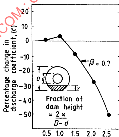
Figure 12 — Effect of debris in meter tube (on both sides of plate)
