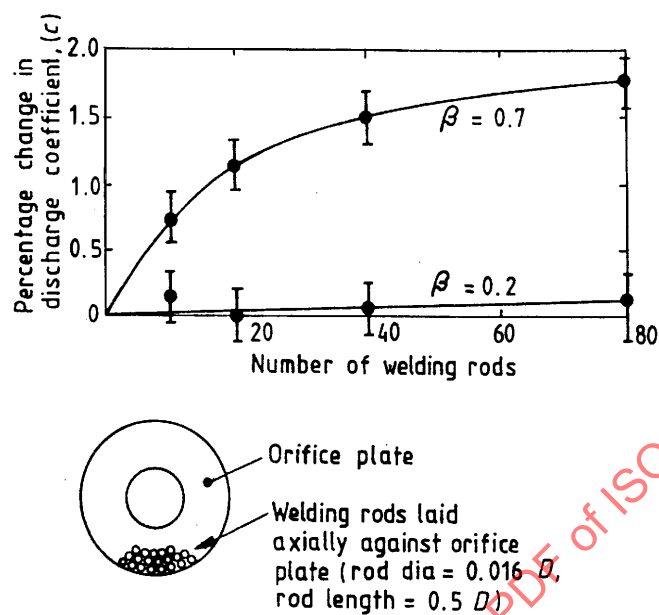
Figure 11 — Effect of welding rods in meter tube
