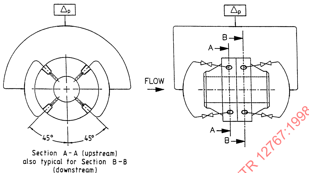
Figure 7 — Triple-T arrangements
