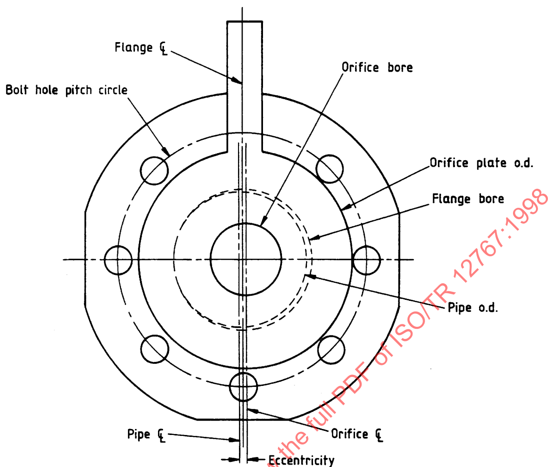
Figure 5 — Possible orifice plate eccentricity resulting from specified tolerances on bolt hole, bolt hole pitch circle, pipe o.d. and flange bore
