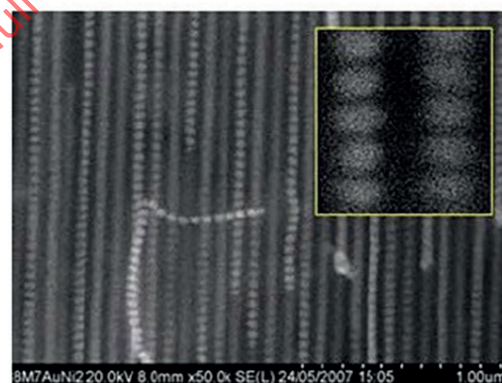
(a) Solutions of gold-silver alloy particles (per-cent of gold content) (b) Scanning electron micrograph of barcode nanowires (multi-segmented nanowires)
