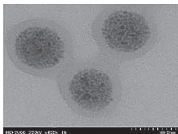
Figure A.1 — Example of oxide nanomaterials – Transmission electron micrograph of aggregated iron oxide particles (based on Figure A.5 from Reference [354]) Image courtesy of National Research Council Canada
