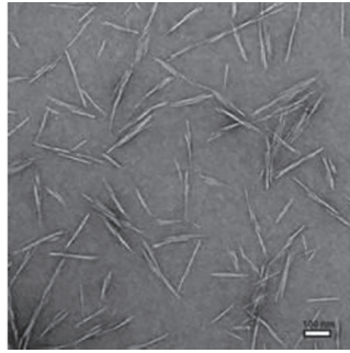
Figure A.4 — Example of cellulose nanomaterials — TEM image of cellulose nanocrystal (CNC) derived from wood pulp (based on Figure 1, from Reference [391]). Image courtesy of National Research Council Canada
