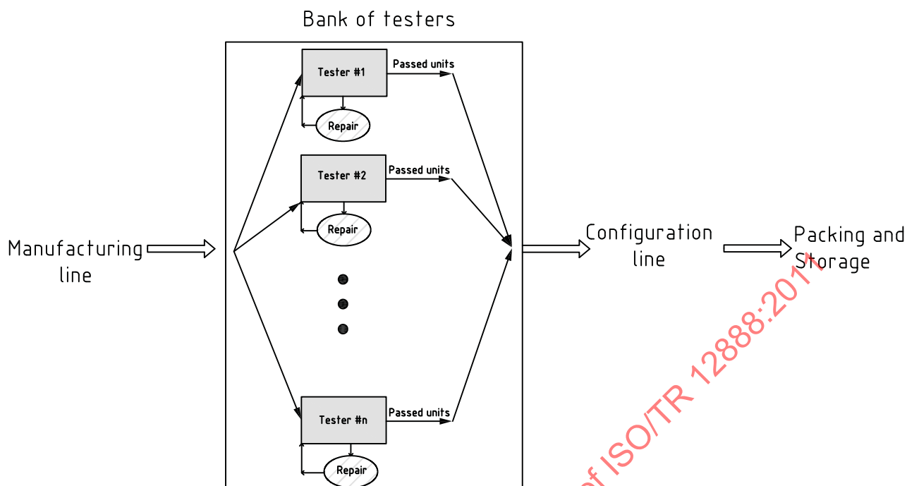
Figure A.1 — Testing process for cell phones
