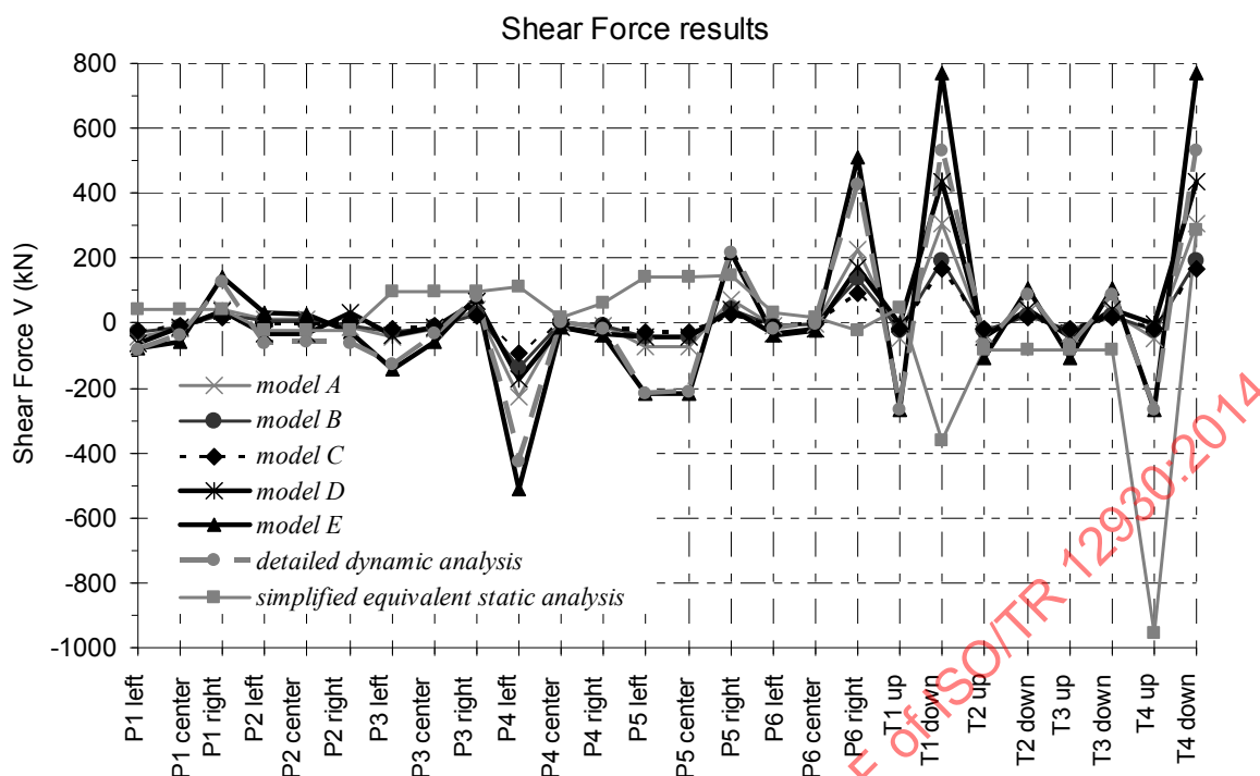
Figure 173 — Shear forces at the cross-section for various analysis cases. Models A to E correspond to equivalent static analysis with imposed quasi static seismic ground deformations displacements at the side boundaries of the FE mesh.
