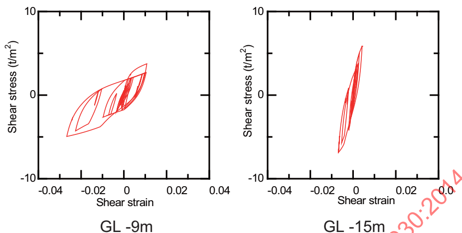
Figure 127 — Relations between response shear stress and shear strain at two different depths
