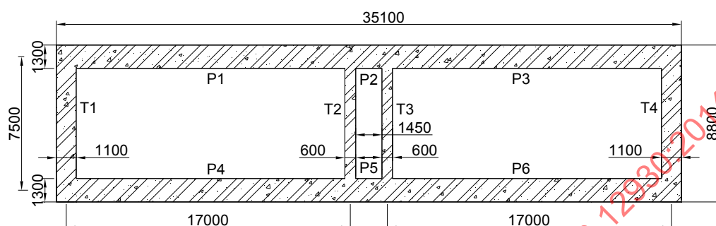
Figure 162 — Simplified tunnel cross-section
