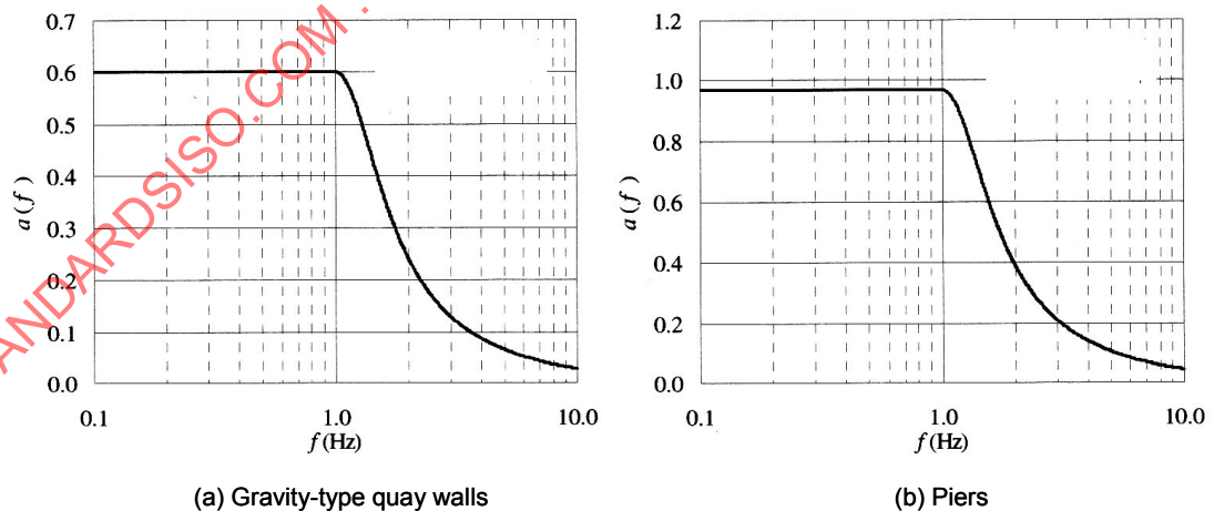
Figure 113 — Filter to consider the effect of frequency
