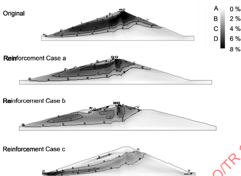
Figure 105 — Maximum shear strain ( \gamma_{\max} ) diagrams in case of Kawanishi Wave for input motion
