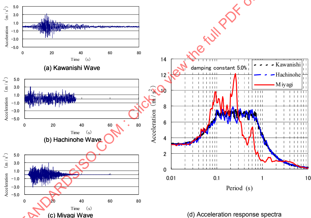
Figure 99 — Acceleration time histories for design input motions and acceleration response spectra of the motions
