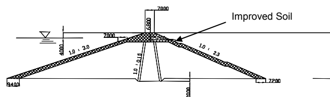
(c) Reinforcement Case c
