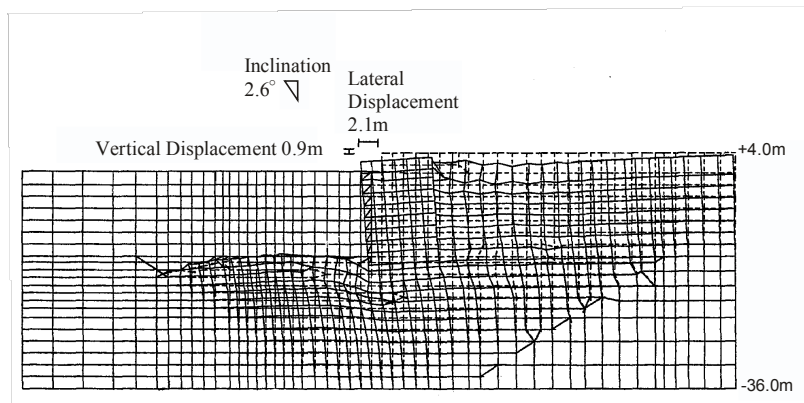
(a) Alternative case 4
