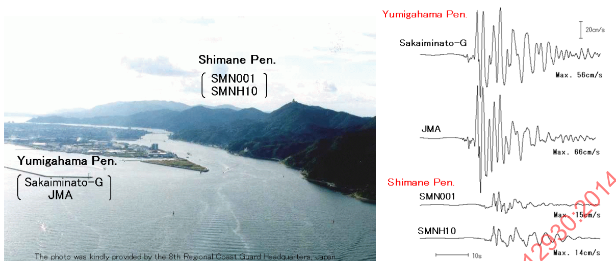
Figure 30 — The topography around the Port of Sakai, western Japan (left) and the velocity waveforms for the fault-normal component recorded around the port during the 2000 Tottori-ken Seibu earthquake (MJ7.3). The peak ground velocities observed in the plains of Yumigahama Peninsula were approximately four times larger than those observed in mountainous Shimane Peninsula (Nozu et al., 2008).
