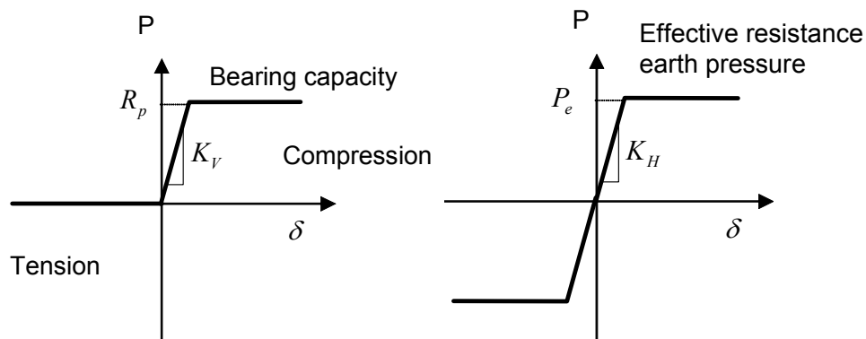
(a) Vertical spring at pile toe
