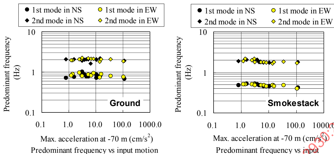
Figure 154 — Relationship between the predominant frequencies and the magnitude of the input in the systems of the ground and the smokestack
