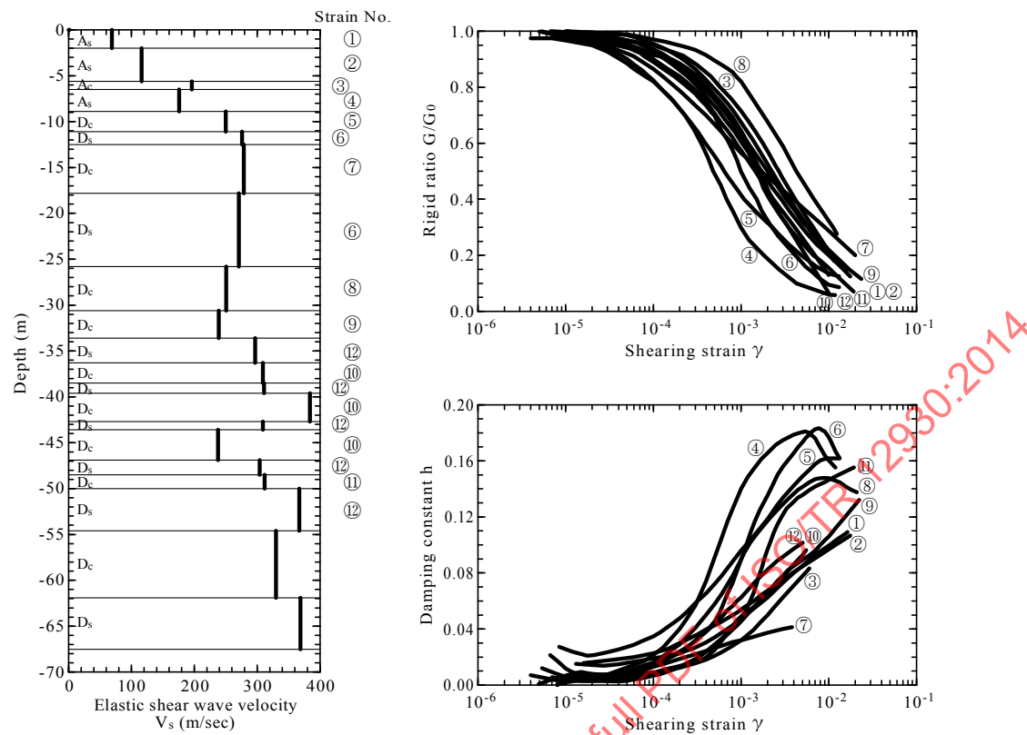
Figure 67 — Soil profile and strain-dependent characteristics
