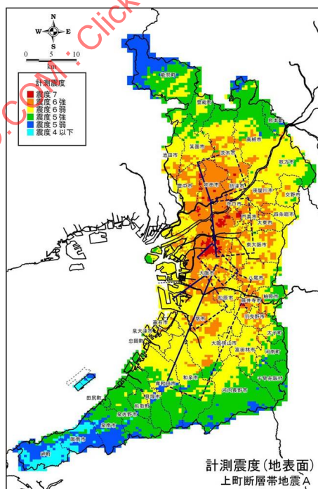
Figure 28 — Distribution of JMA seismic intensity caused by a scenario earthquake, the Uemachi fault A (Osaka Prefecture, 2007)
