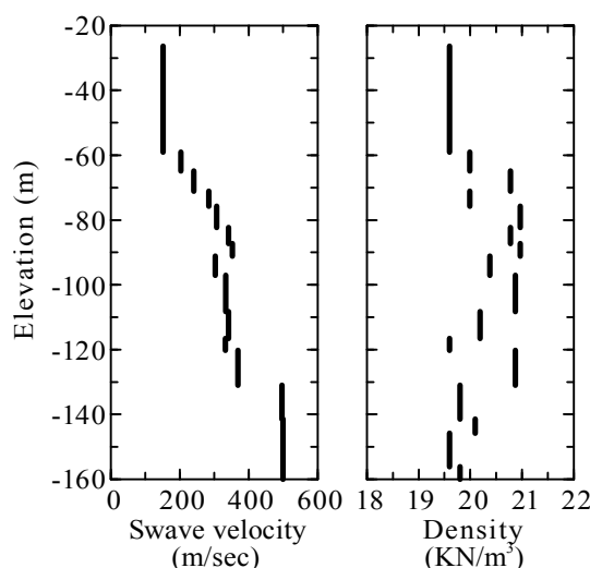
Figure 86 — Soil profile [1]
