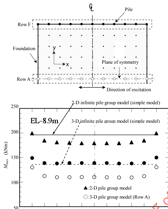
Figure 182 — Maximum bending moment of each pile
