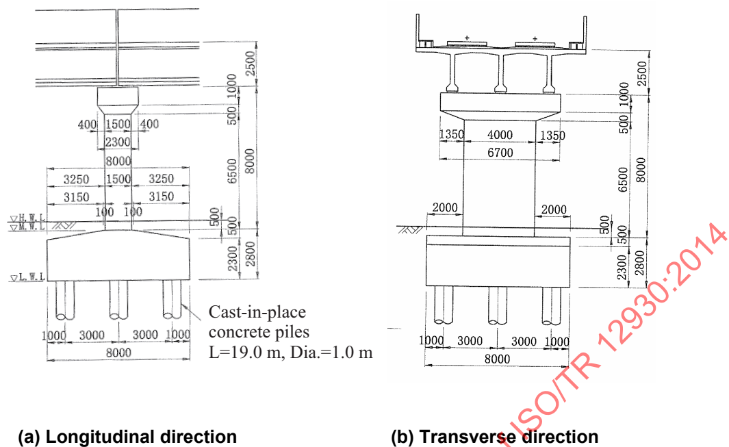
Figure 117 — Reinforced concrete bridge pier (Unit: mm when no unit shown)
