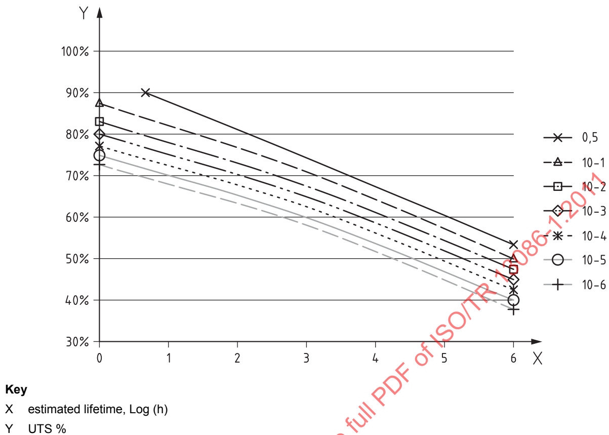
Figure 2 — Maximum likelihood estimates of lifetimes of aramid/epoxy for vessels, with quantile probabilities
