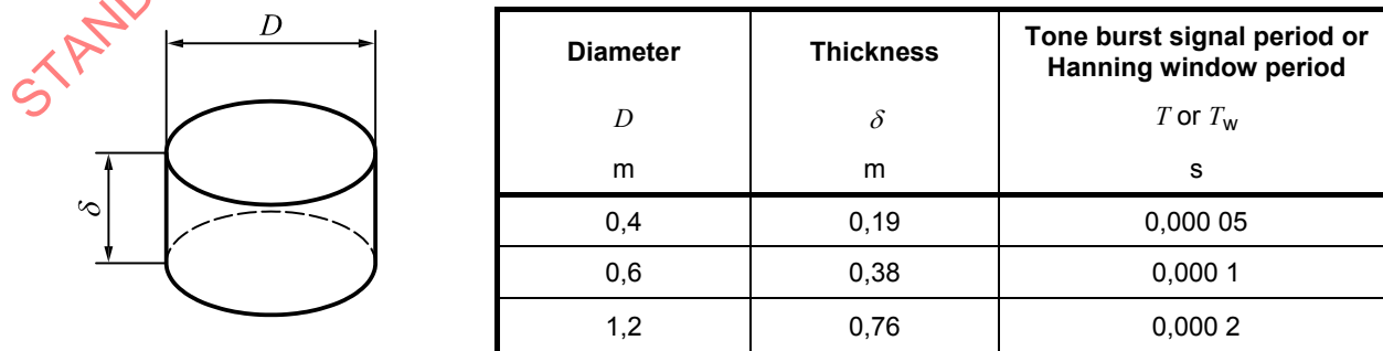
Figure 1 — Dimension of transfer medium and setting of period T or T_w
