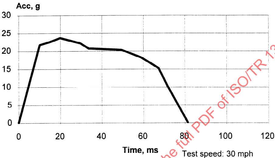
Frontal impact FMVSS 213, configuration I
